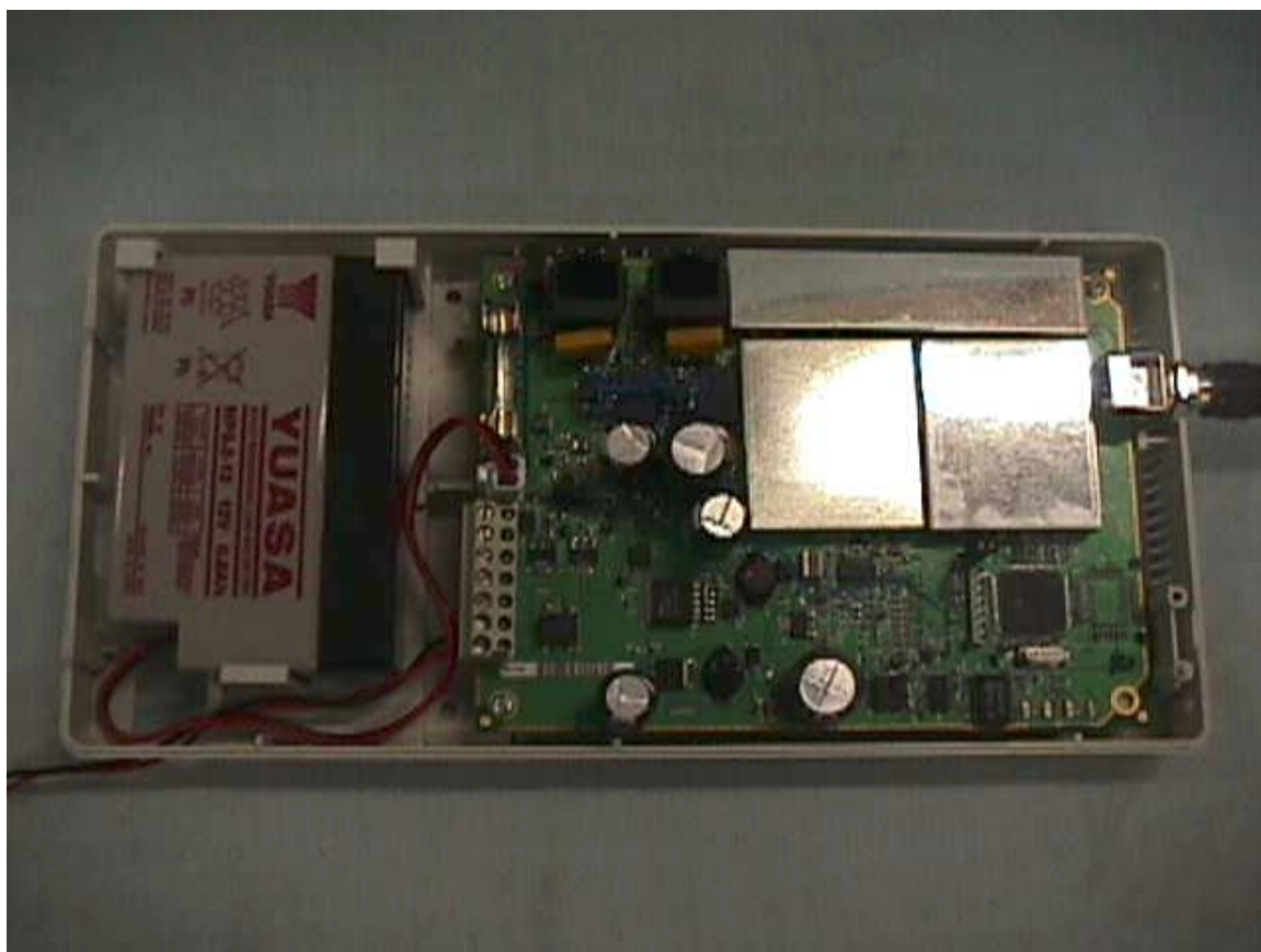
Assembly – T100C001
