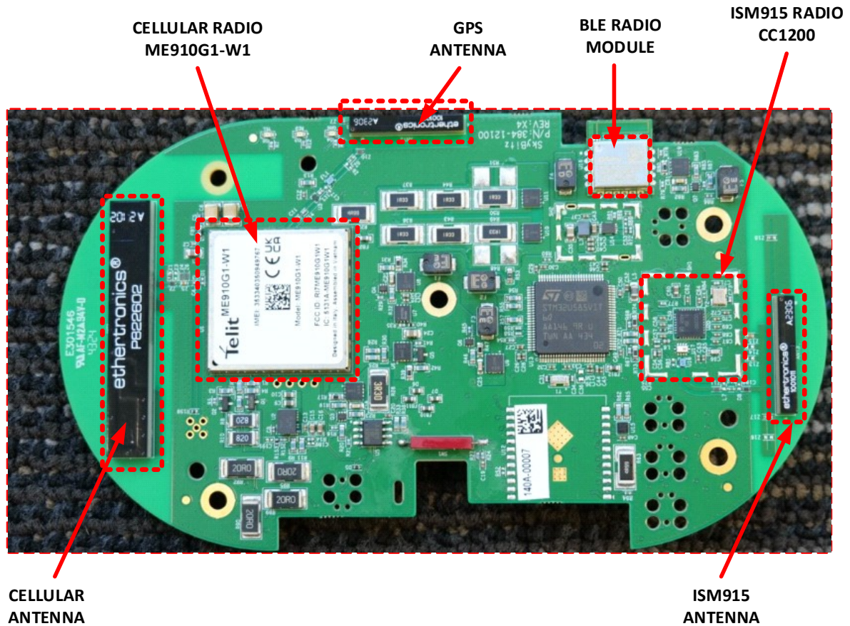
Top Side of Printed Circuit Board Assembly
