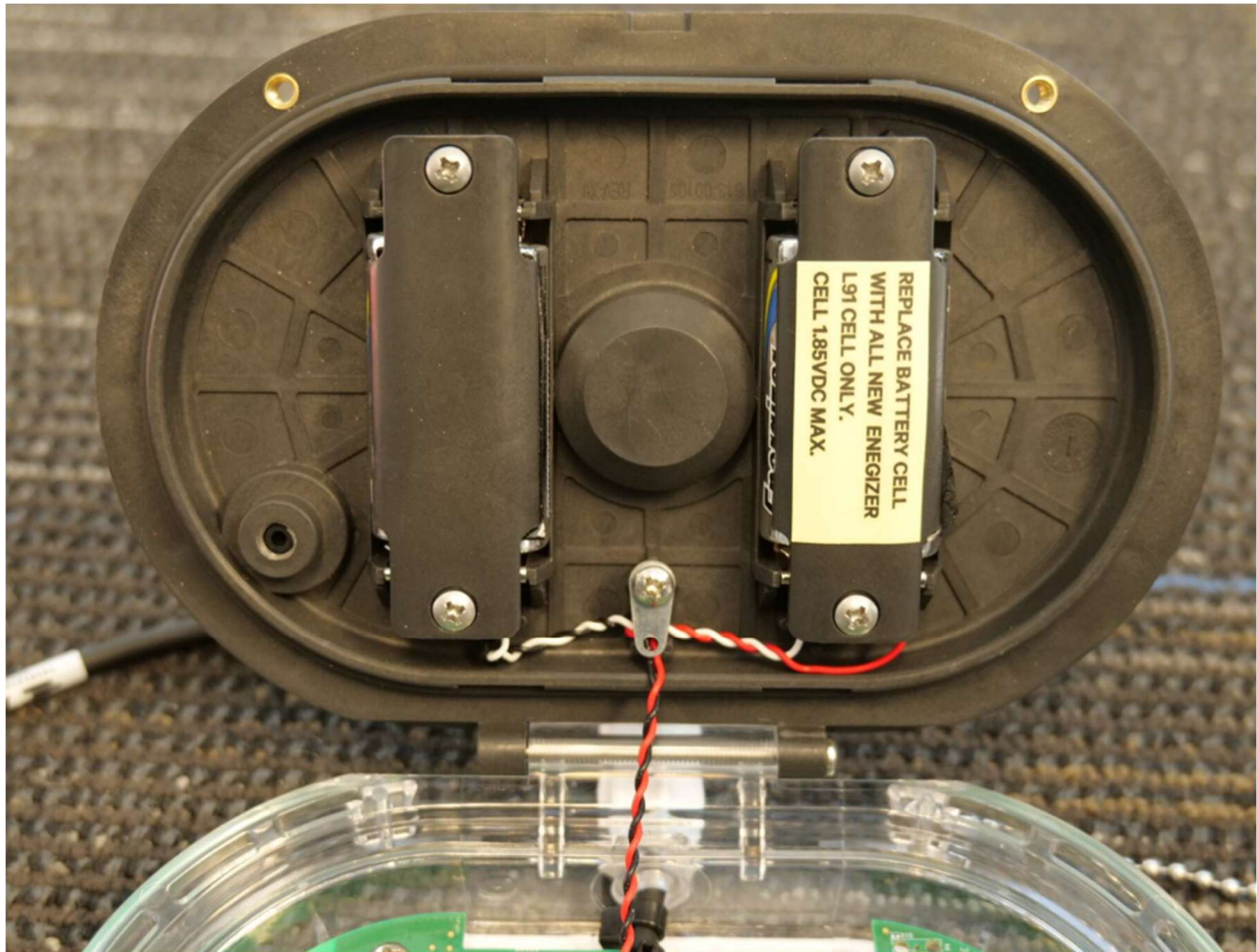
Top Internal Closeup View Showing Battery Cell Securement
