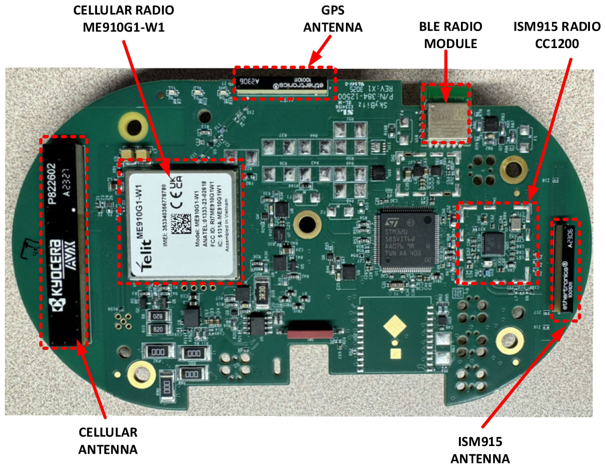
Top Side of Printed Circuit Board Assembly
