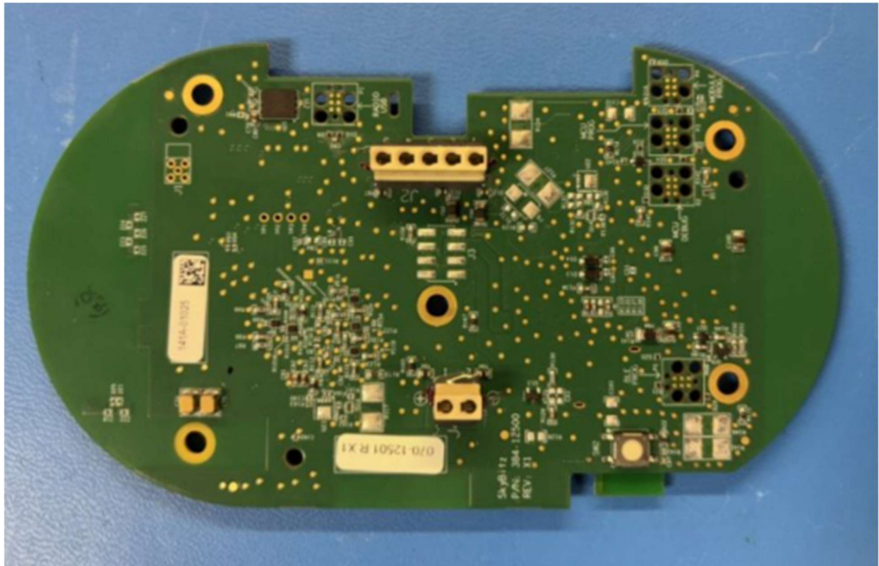
Bottom Side of Printed Circuit Board Assembly
