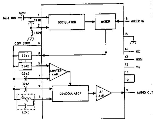
Figure 4-3 U241 BLOCK DIAGRAM
