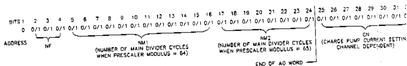
Figure 3-3 A-WORD
