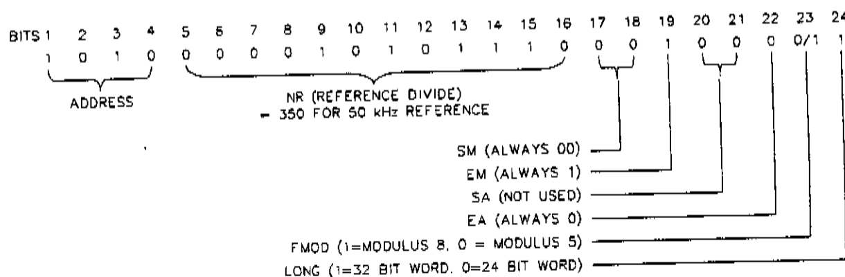
Figure 3-1 D-WORD
