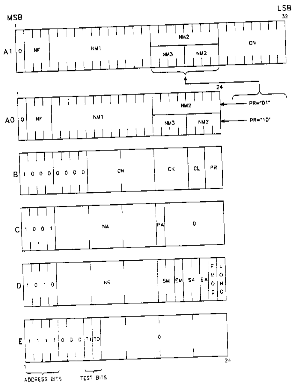
Figure 3-4 SERIAL INPUT WORD FORMAT
