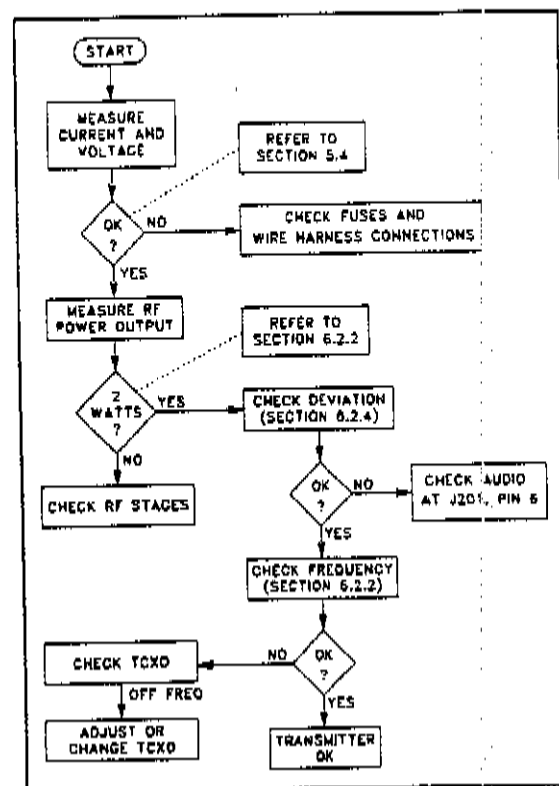
Figure 5-2 TRANSMITTER SERVICING FLOWCHART
