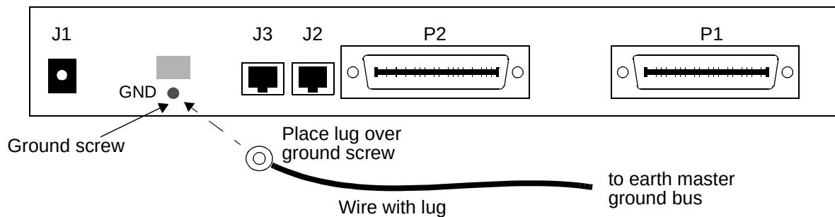
Figure 3-9. CTPhone Controller Ground Requirements
