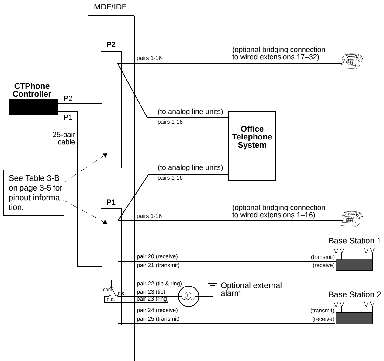
Figure 3-1. Overview of CTPhone 1900 System Cabling
