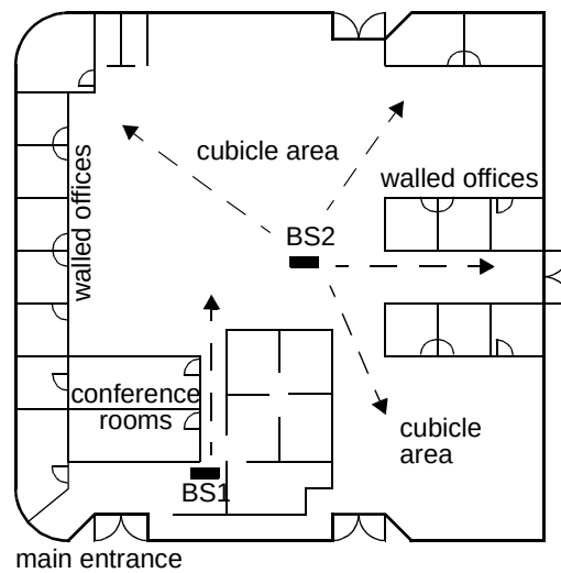
Figure 2-14. Base Station Placement in Office Environment
