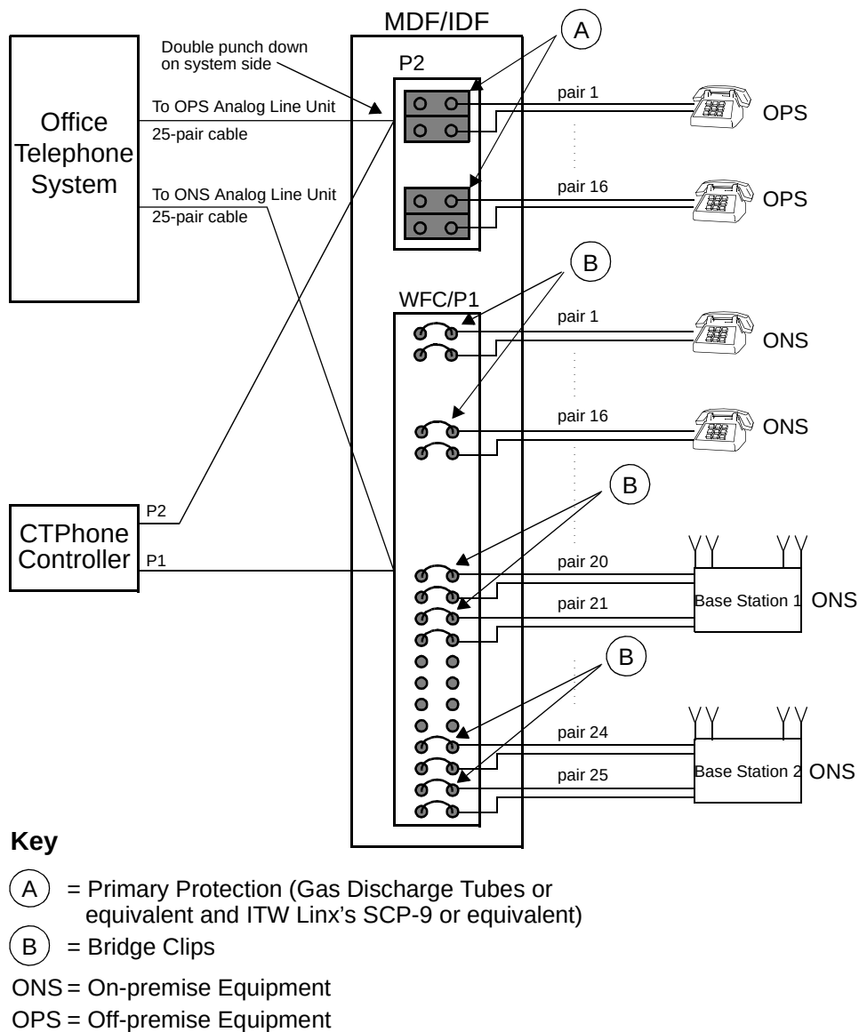
Figure A-1. Primary and Secondary Protectors
