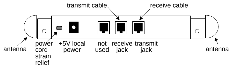
Figure 3-5. Base Station Connections
