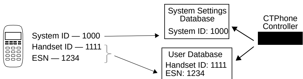
Figure 4-2. Relationship Between ESN, System ID, & Handset ID
