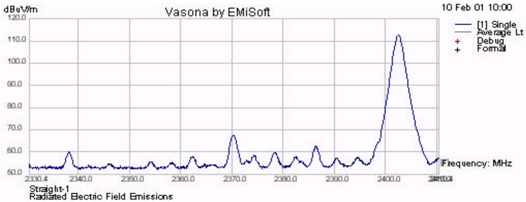
Band-edge Measurement, Low Channel
