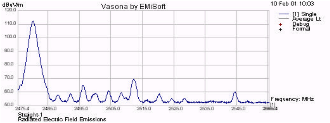
Band-edge Measurement, High Channel
