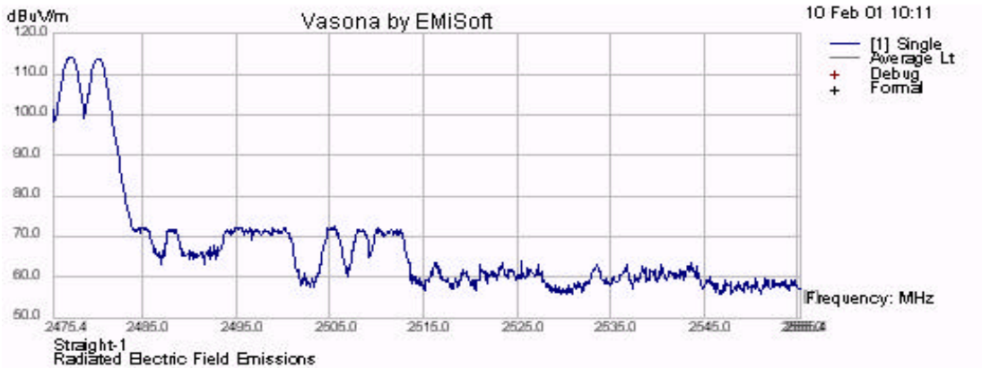
Band-edge Measurement, High Channel, Freq. Hopping Mode
