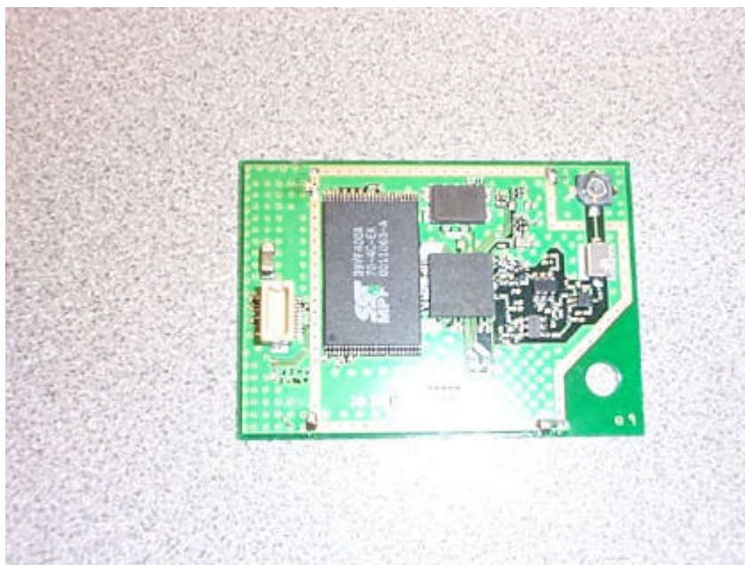
EUT: FPCWL02 Radio Portion with Shield Removed(1)
