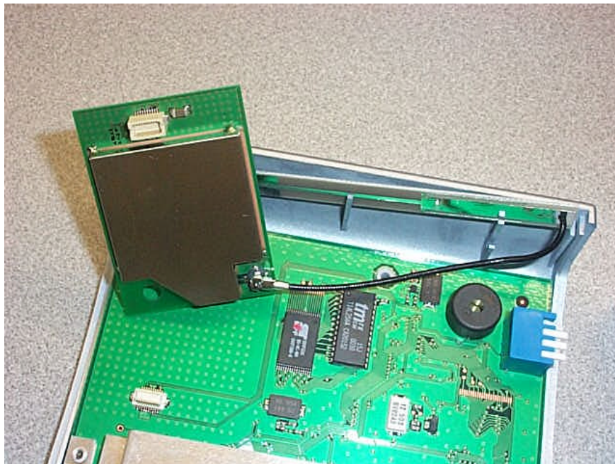
EUT: FPCWL02 Internal(3)
