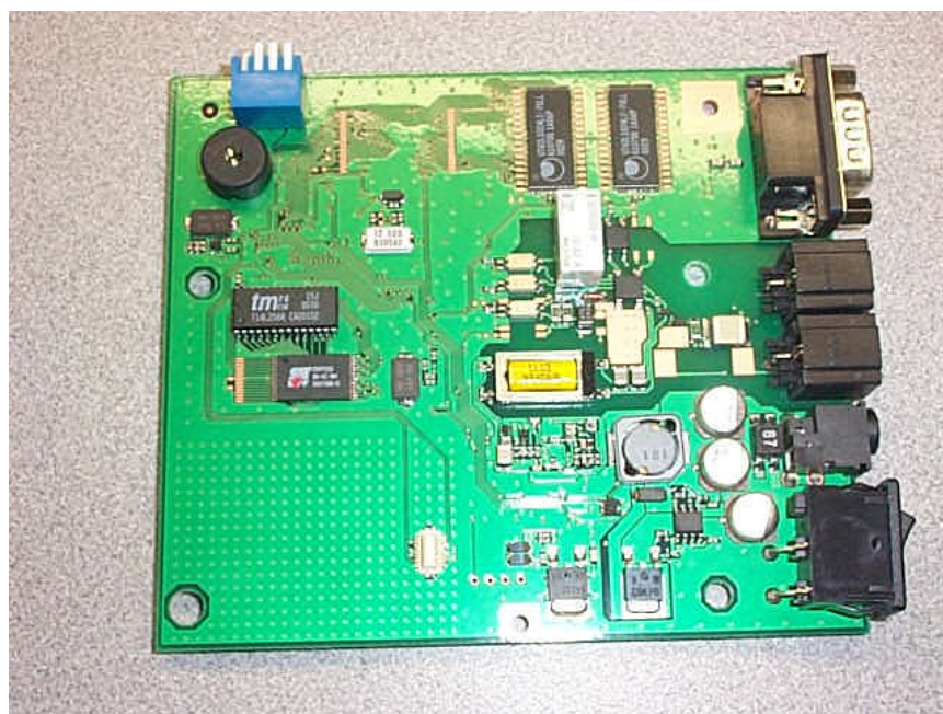
EUT: FPCWL02 Internal with Heatsink Removed (4)
