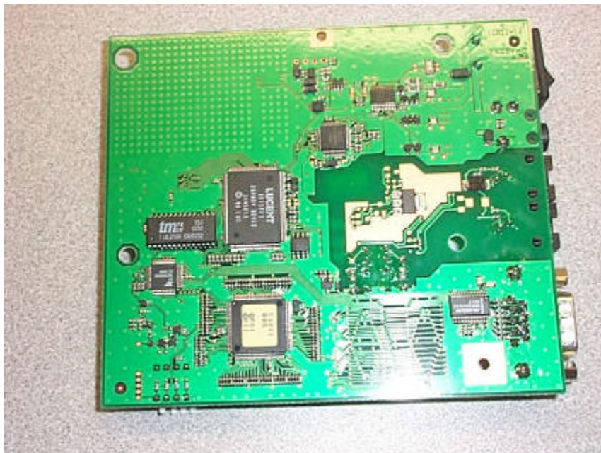
EUT: FPCWL02 Internal(5)
