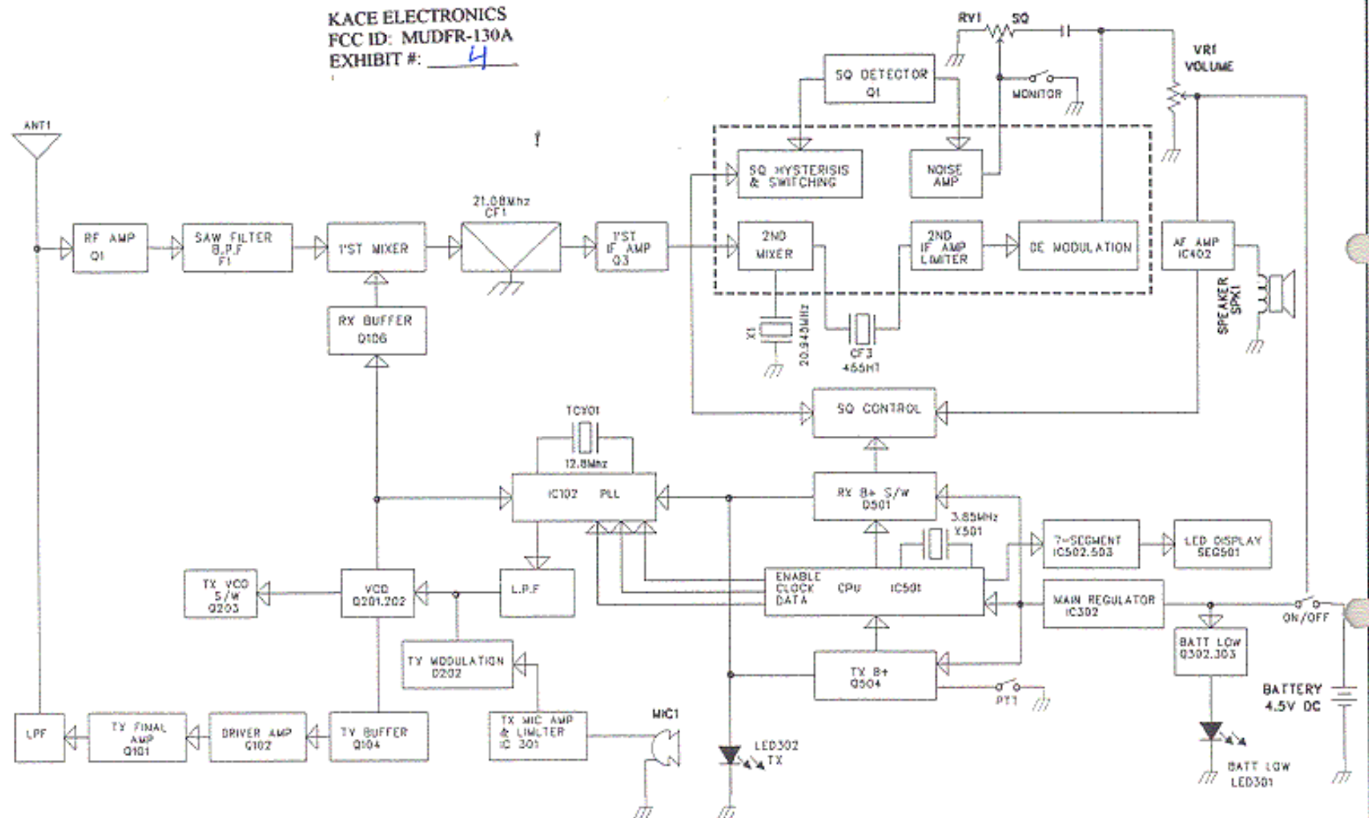
FR-130A BLOCK DIAGRAM
