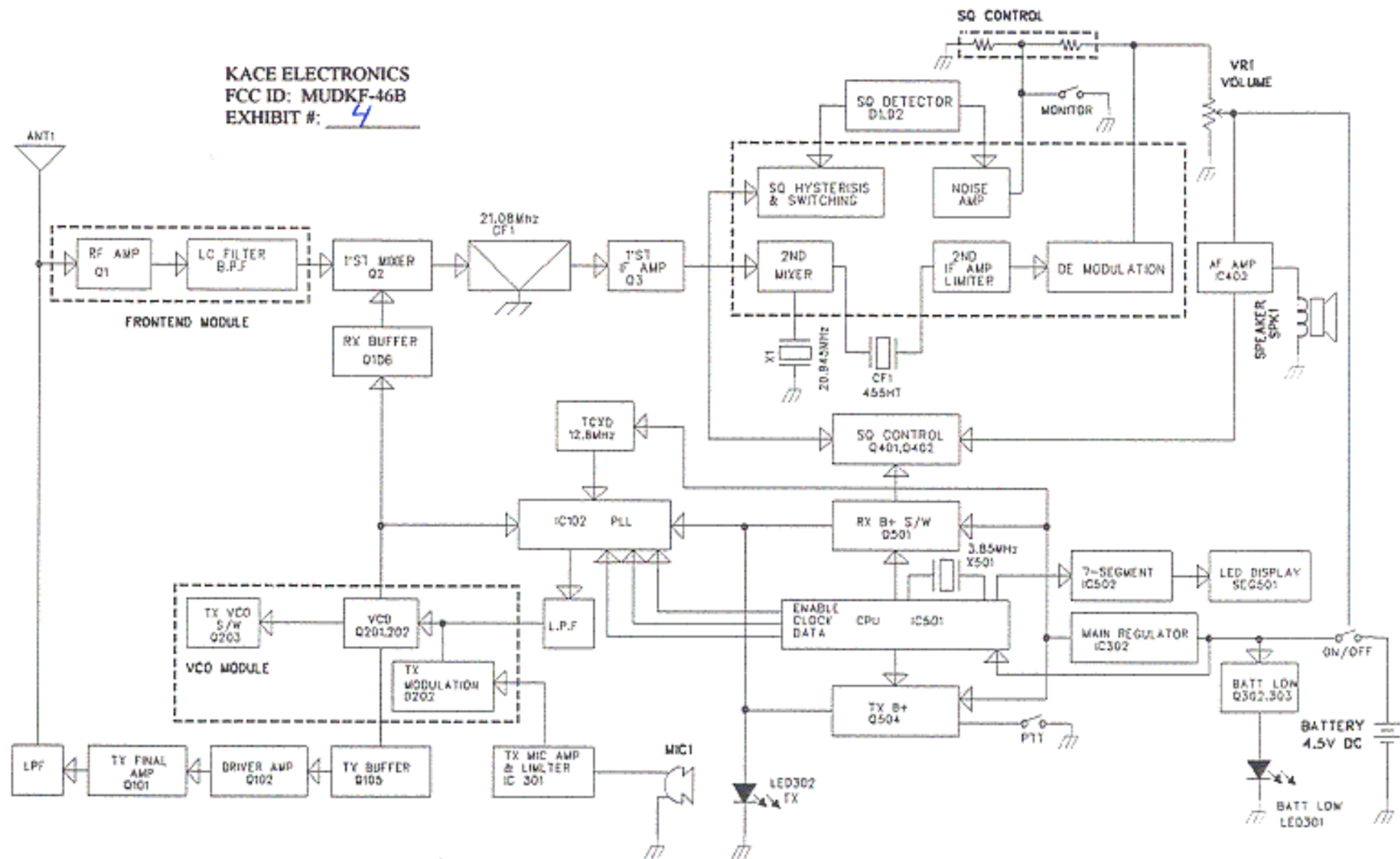
GE3-5870B BLOCK DIAGRAM
