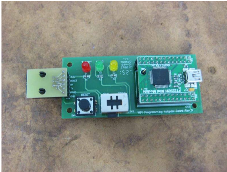
USB to Serial Module
