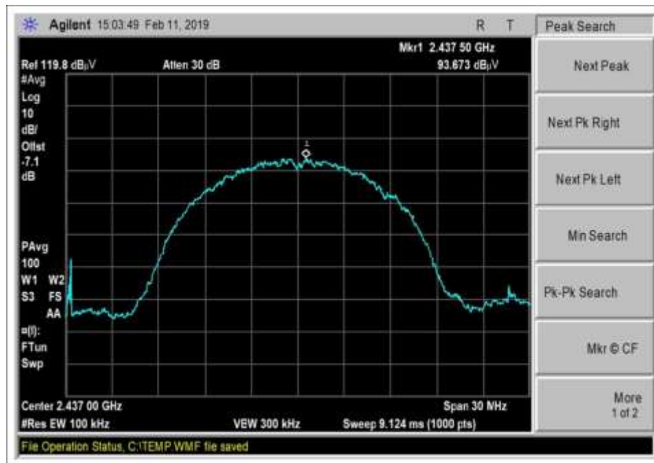
Middle Channel_b_11Mbps
