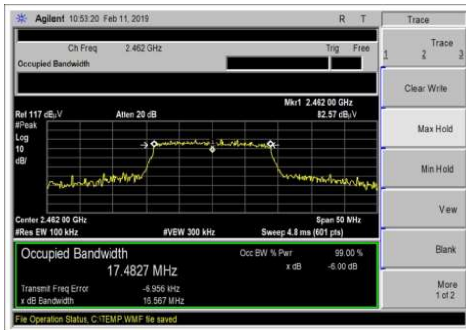
High Channel_n20_MCS7
