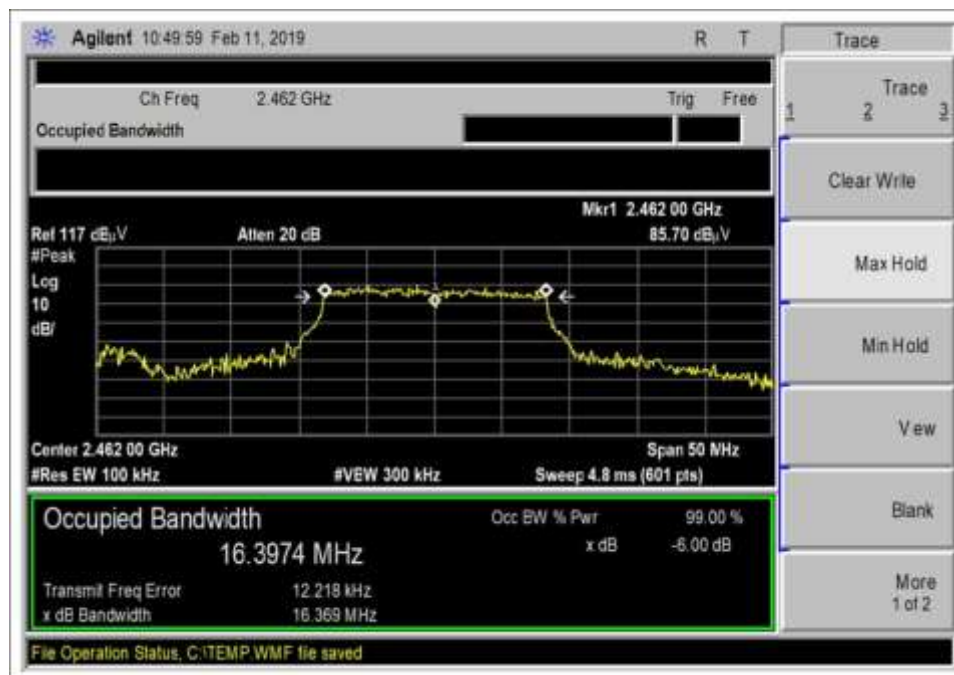
High Channel_g_54Mbps
