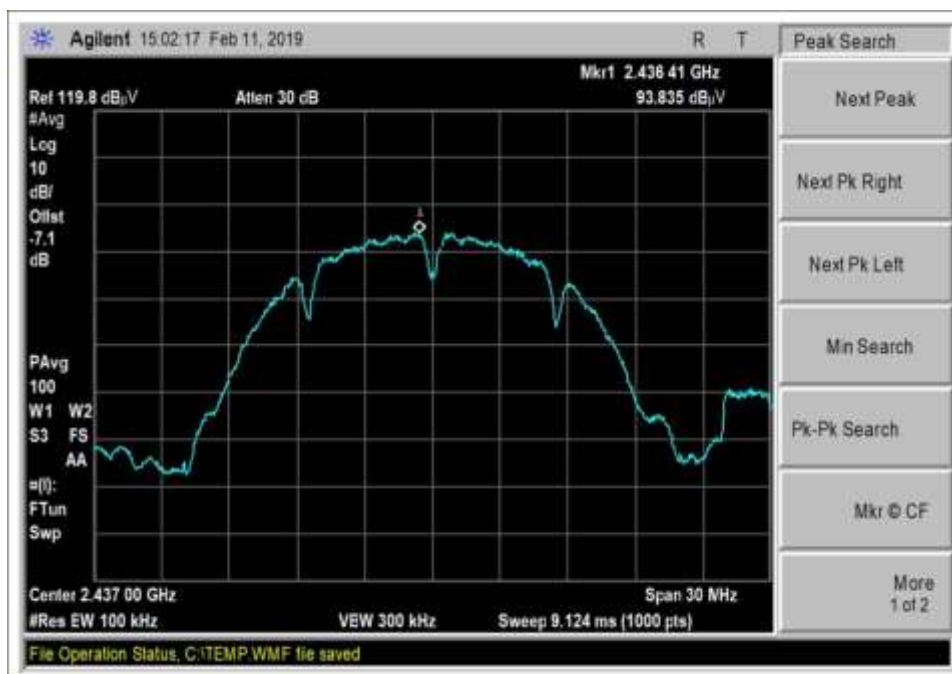
Middle Channel_b_1Mbps
