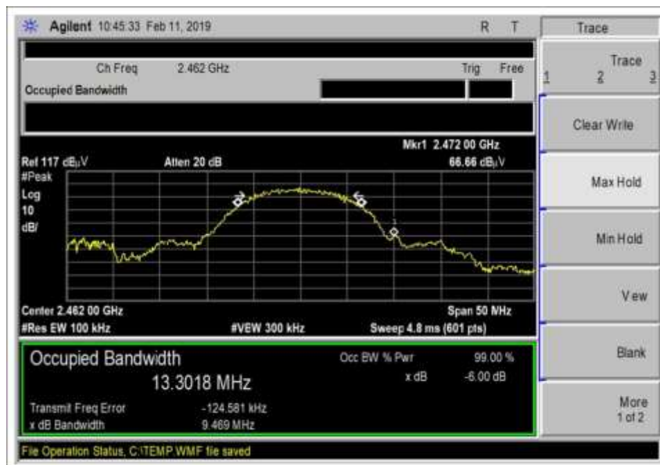
High Channel_b_11Mbps
