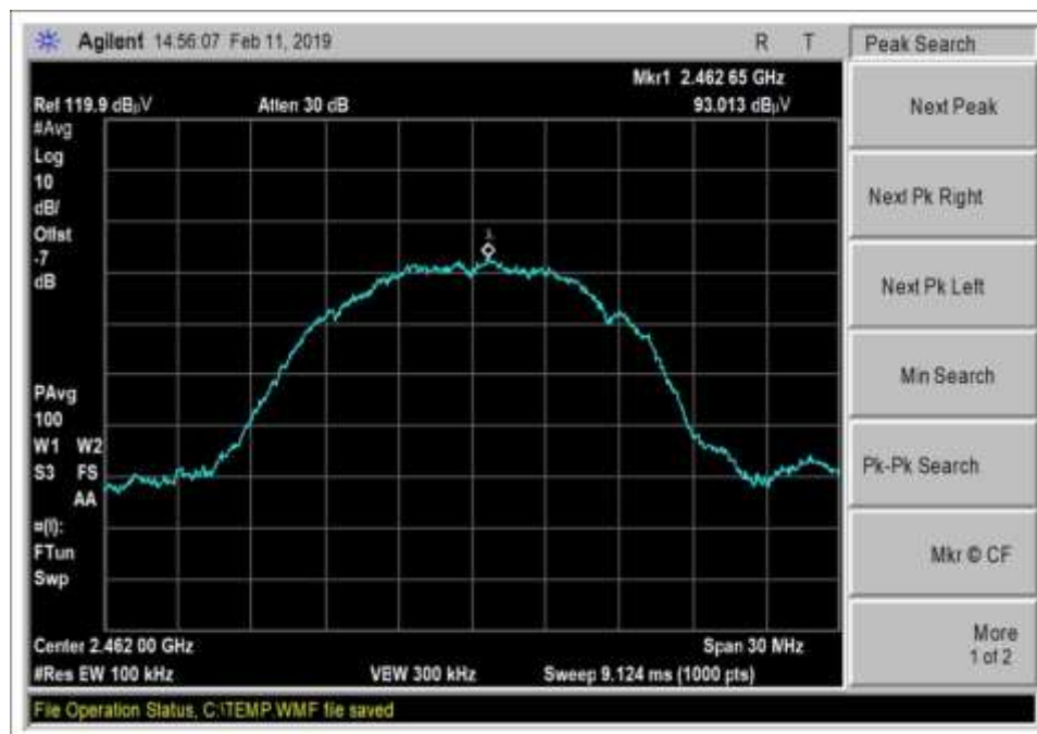
High Channel_b_11Mbps
