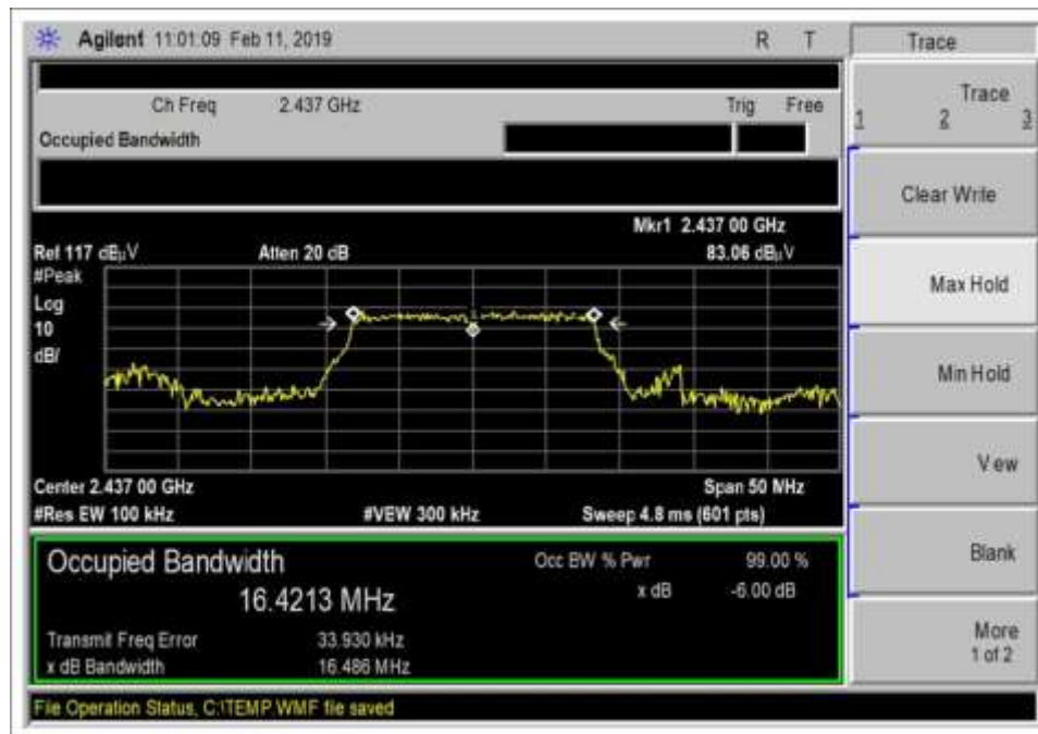
Middle Channel_g_54Mbps
