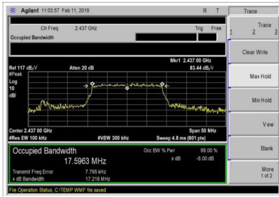
Middle Channel_n20_MCS7
