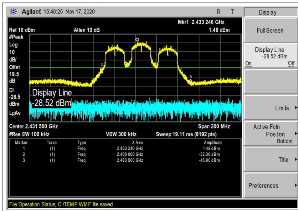
MCS0; 802.11n20
