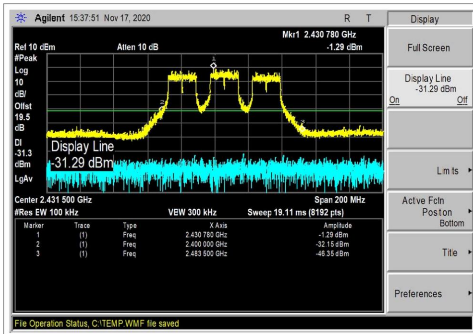
54Mbps; 802.11g
