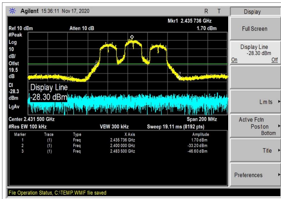
6Mbps; 802.11g
