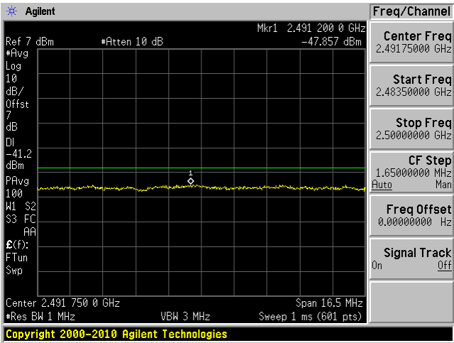
Plot: 2.4835 GHz – 2.5 GHz (restrict band) Ave
