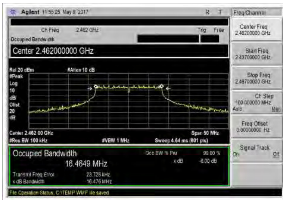
802.11g_High Channel_2462MHz_DTS_-6dB_BW
