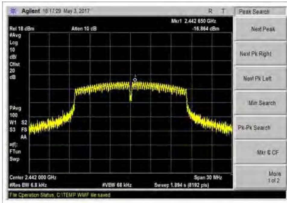
802.11g_Middle Channel_2442MHz_PSD
