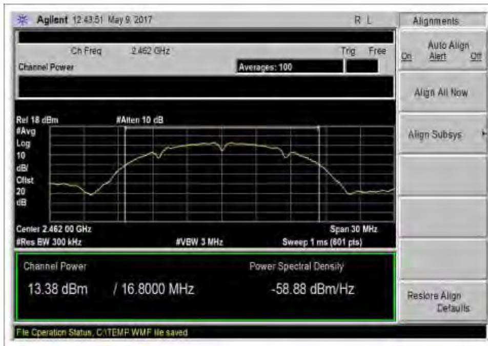
802.11b_High Channel_2462MHz_PowerOutput
