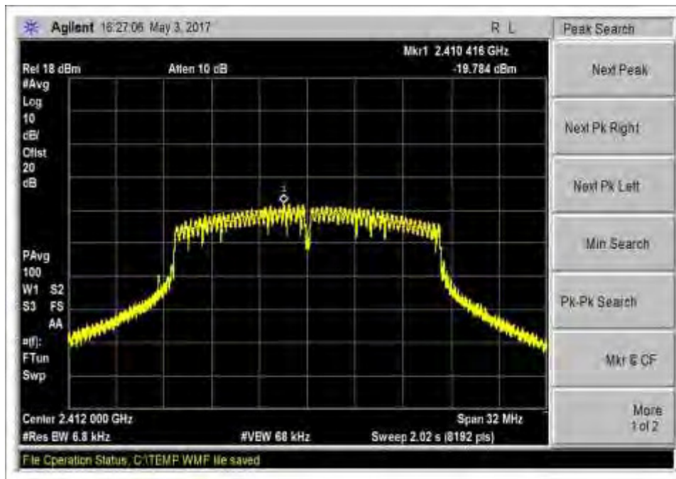
802.11n20_Low Channel_2412MHz_PSD
