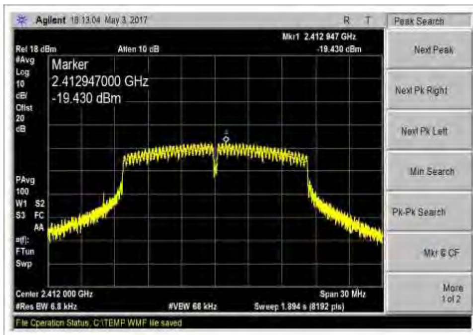
802.11g_Low Channel_2412MHz_PSD
