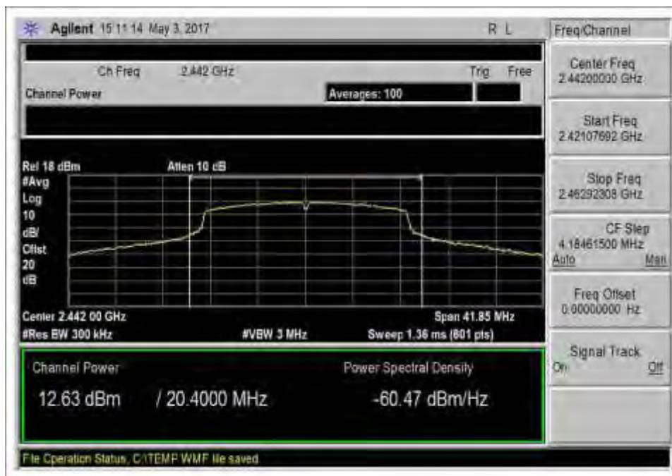
802.11n20_Middle Channel_2442MHz_PowerOutput
