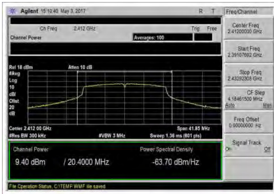
802.11n20_Low Channel_2412MHz_PowerOutput
