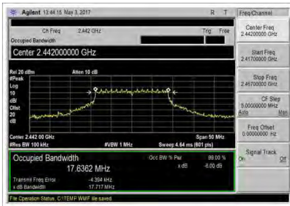
802.11n20_Middle Channel_2442MHz_DTS_-6dB_BW
