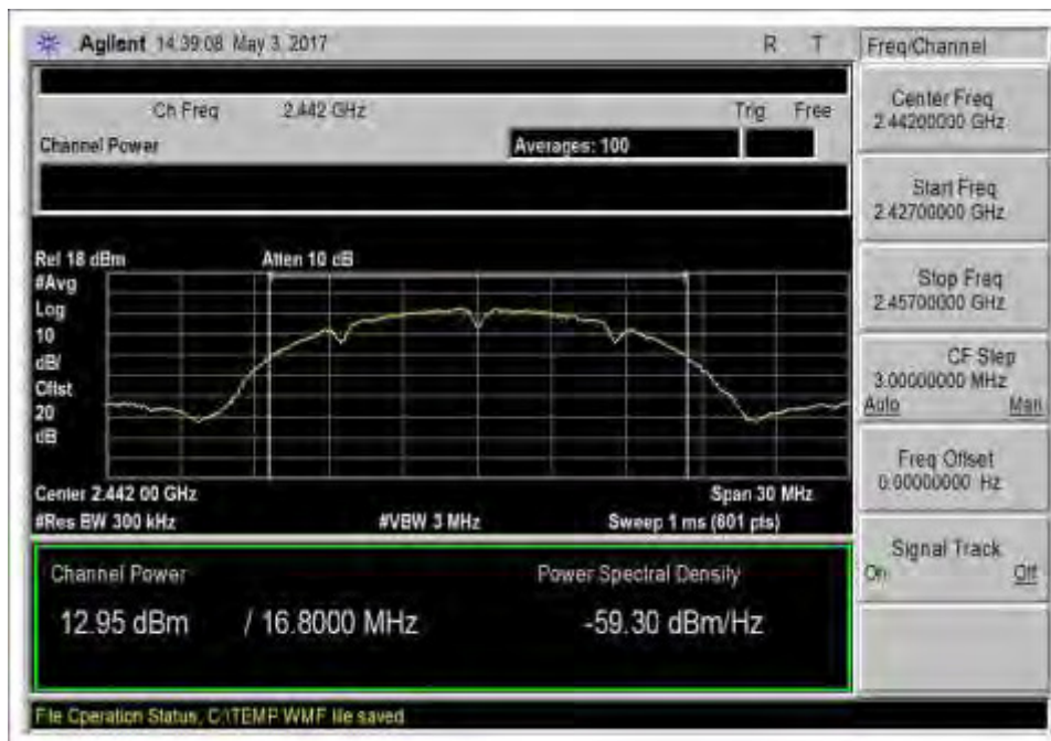
802.11b_Middle Channel_2442MHz_PowerOutput
