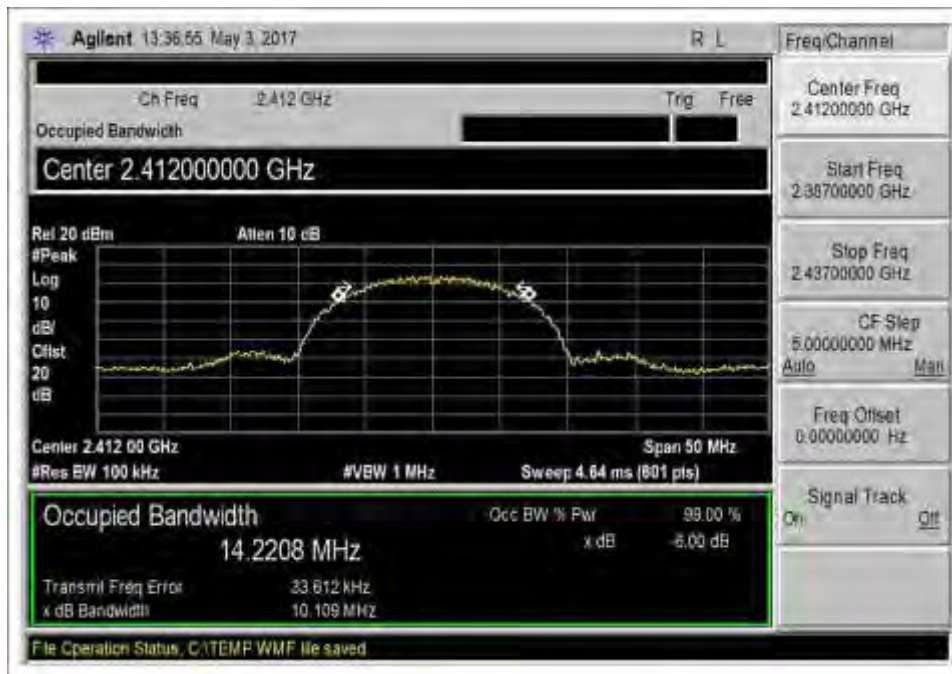
802.11b_Low Channel_2412MHz_DTS_-6dB_BW
