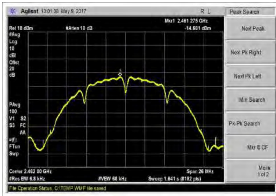
802.11b_High Channel_2462MHz_PSD
