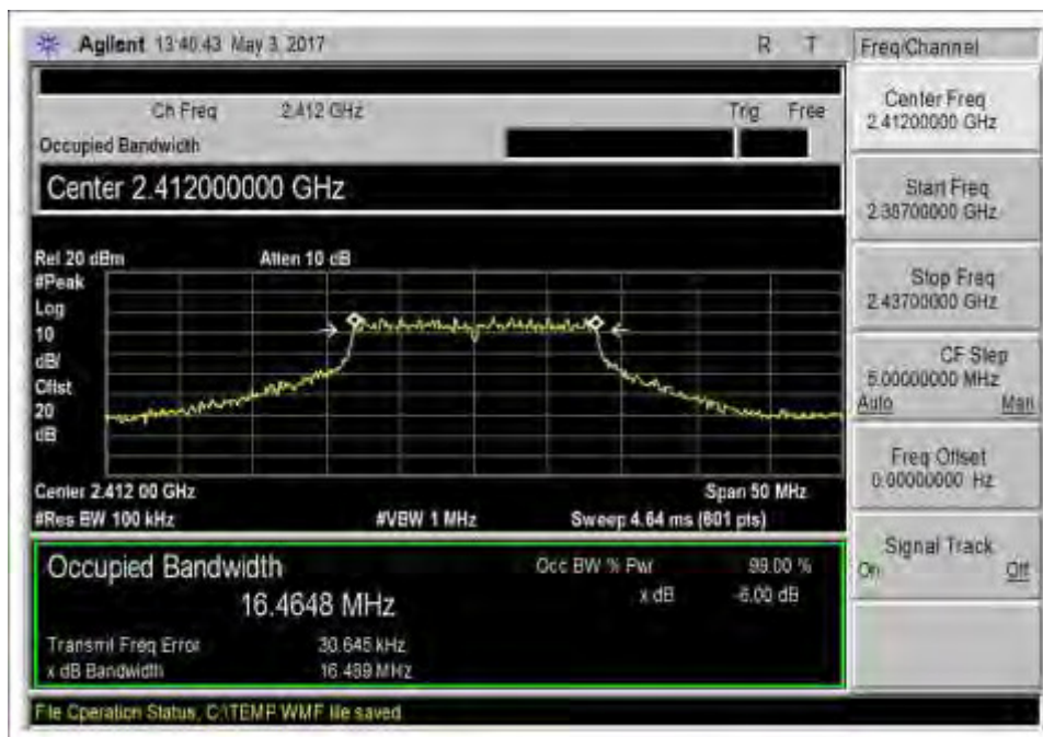
802.11g_Low Channel_2412MHz_DTS_-6dB_BW
