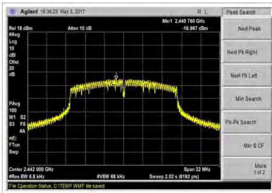
802.11n20_Middle Channel_2442MHz_PSD
