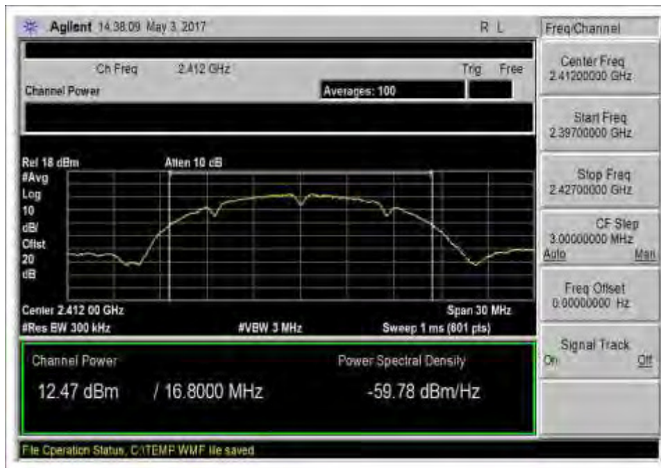
802.11b_Low Channel_2412MHz_PowerOutput
