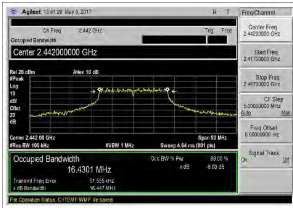
802.11g_Middle Channel_2442MHz_DTS_-6dB_BW
