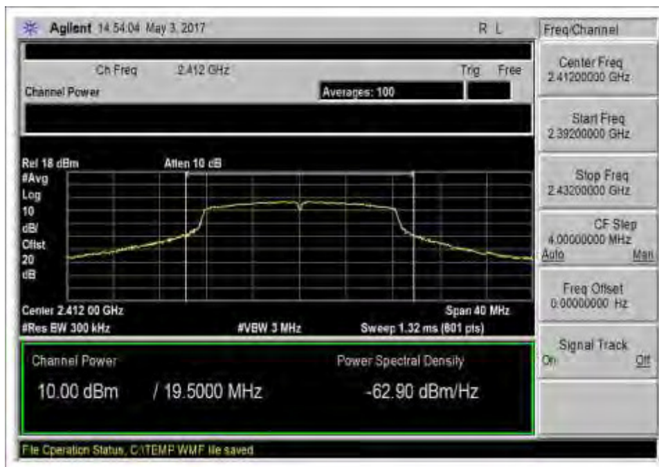
802.11g_Low Channel_2412MHz_PowerOutput
