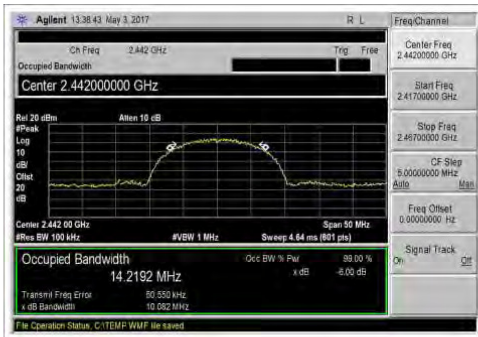
802.11b_Middle Channel_2442MHz_DTS_-6dB_BW
