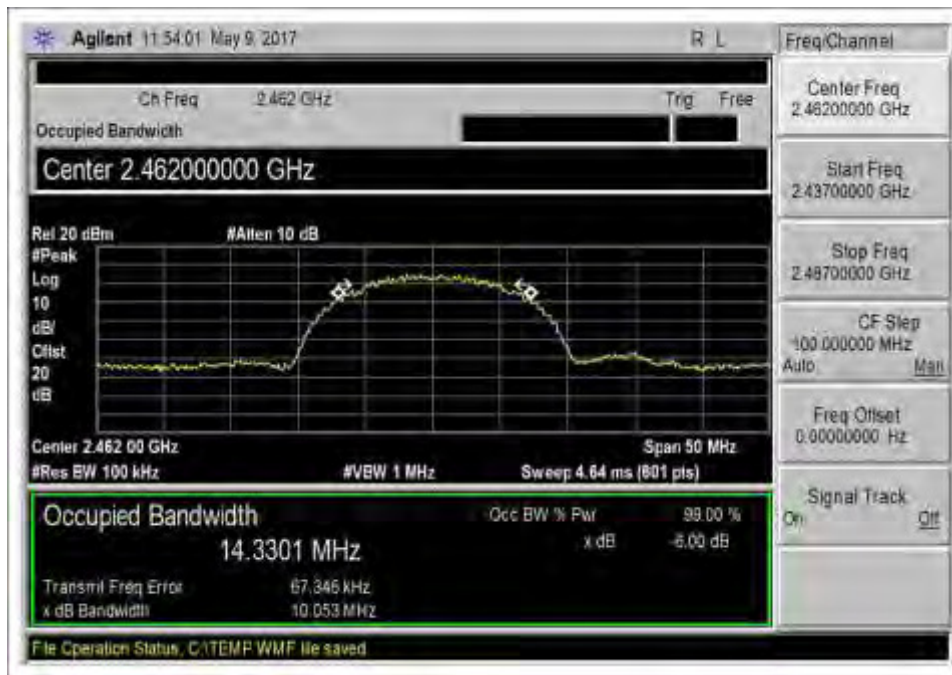
802.11b_High Channel_2462MHz_DTS_-6dB_BW
