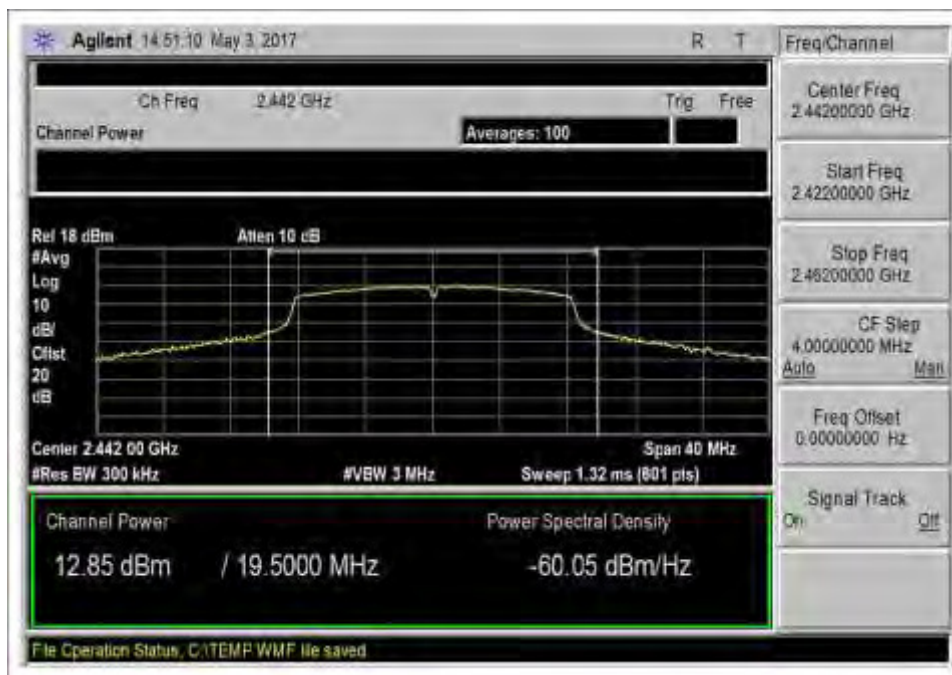
802.11g_Middle Channel_2442MHz_PowerOutput
