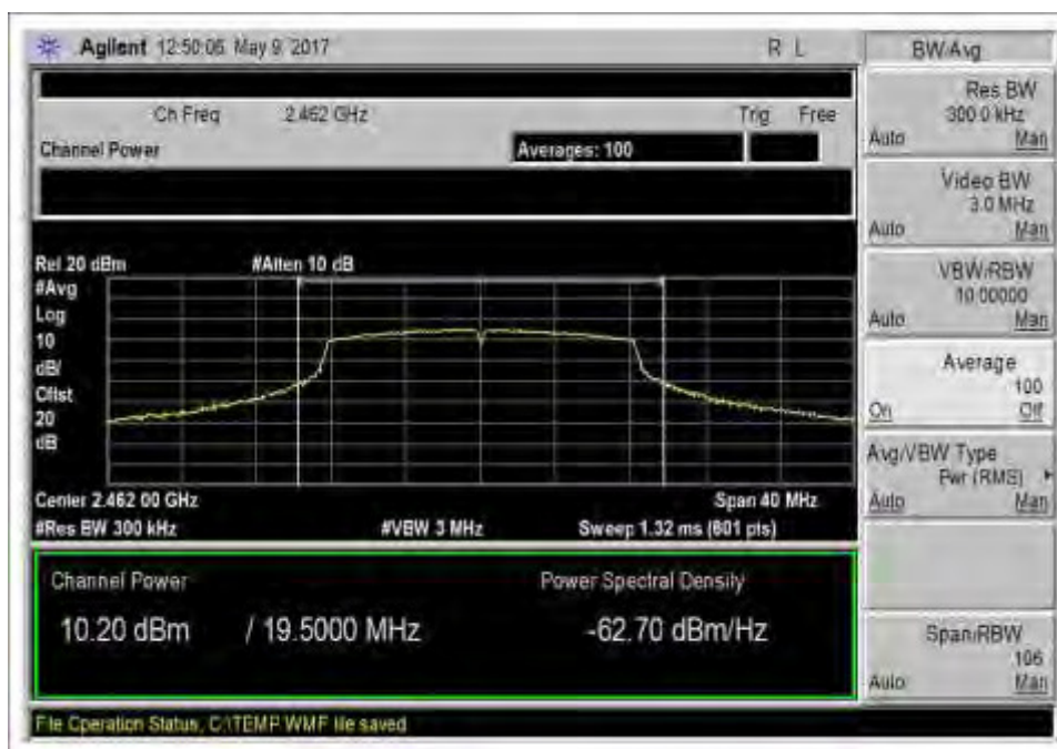
802.11g_High Channel_2462MHz_PowerOutput
