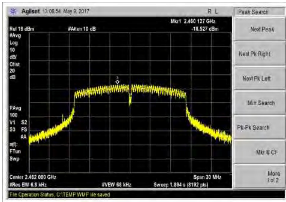
802.11g_High Channel_2462MHz_PSD
