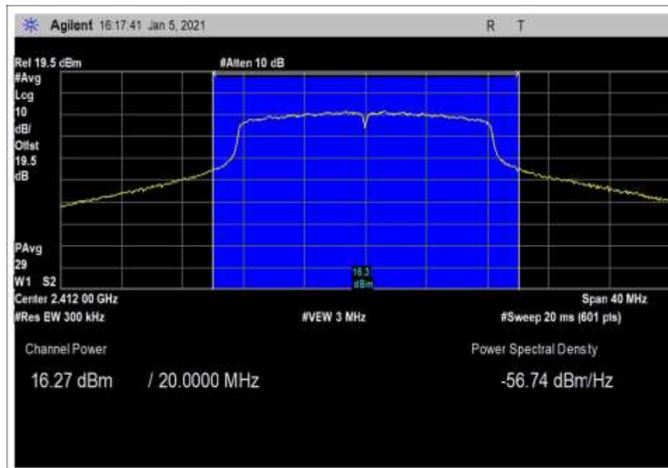
power_802.11g_Low Channel_17dBm
