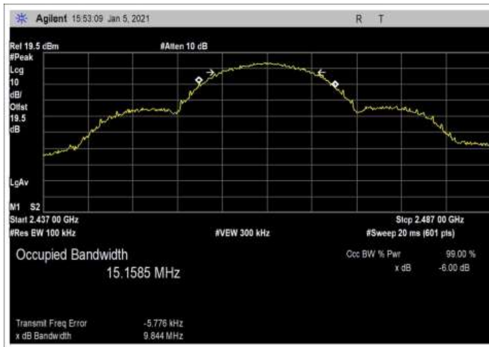
-6dB_BW_802.11b_High Channel_20dBm
