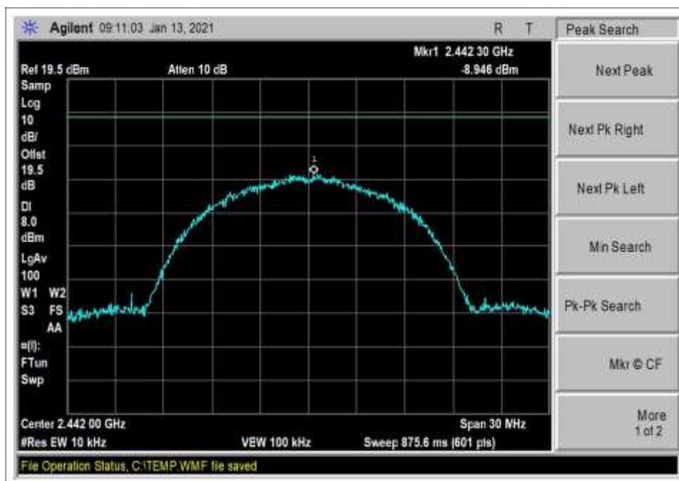
PSD_802.11b_Middle Channel_19dBm
