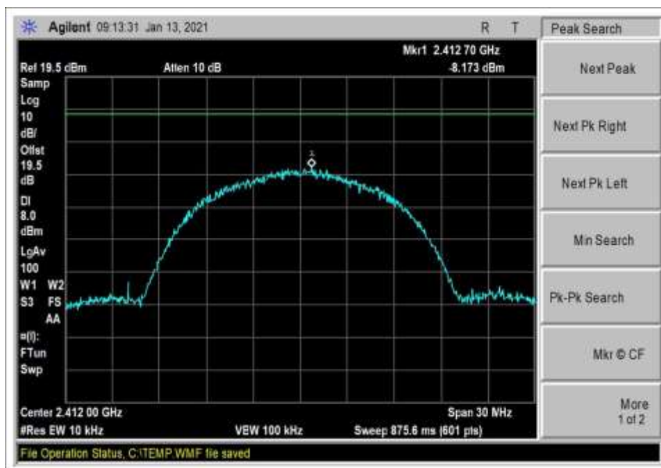
PSD_802.11b_Low Channel_19dBm
