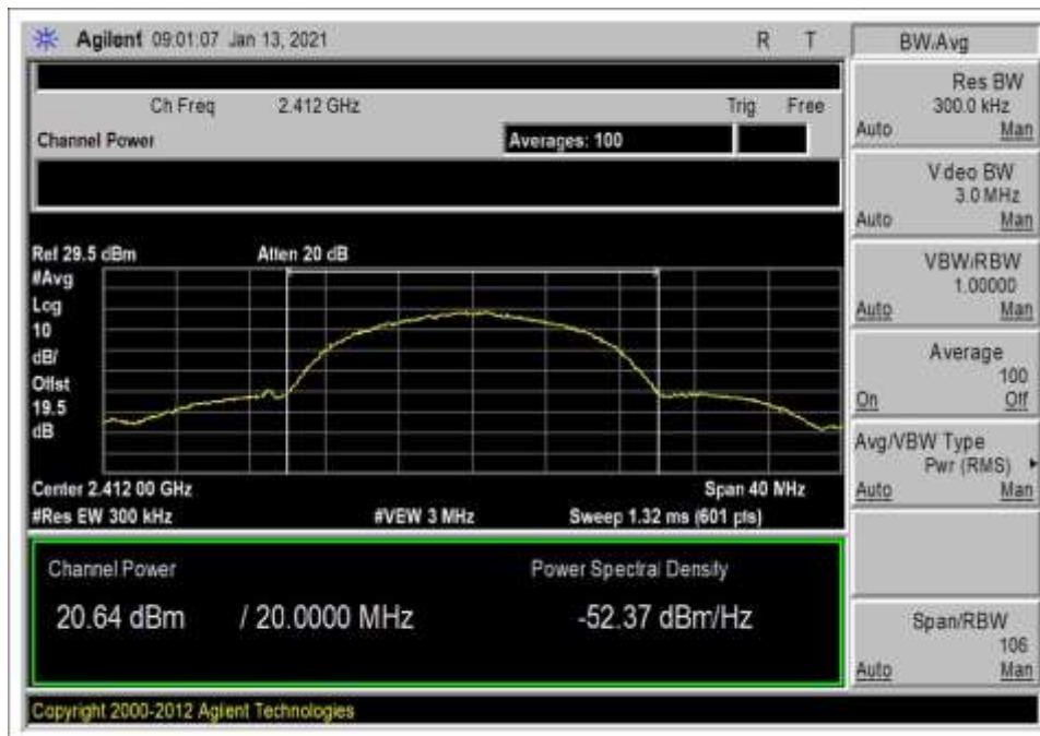
power_802.11b_Low Channel_19dBm
