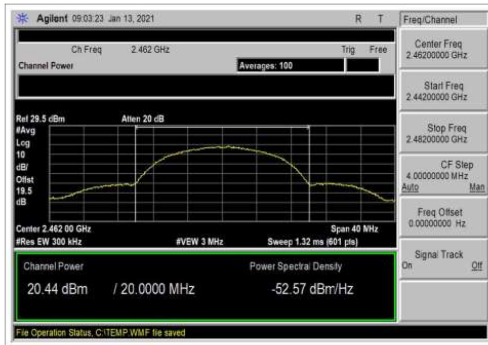
power_802.11b_High Channel_19dBm
