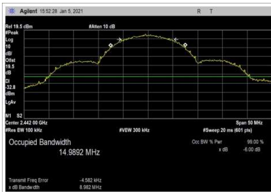
-6dB_BW_802.11b_Middle Channel_20dBm
