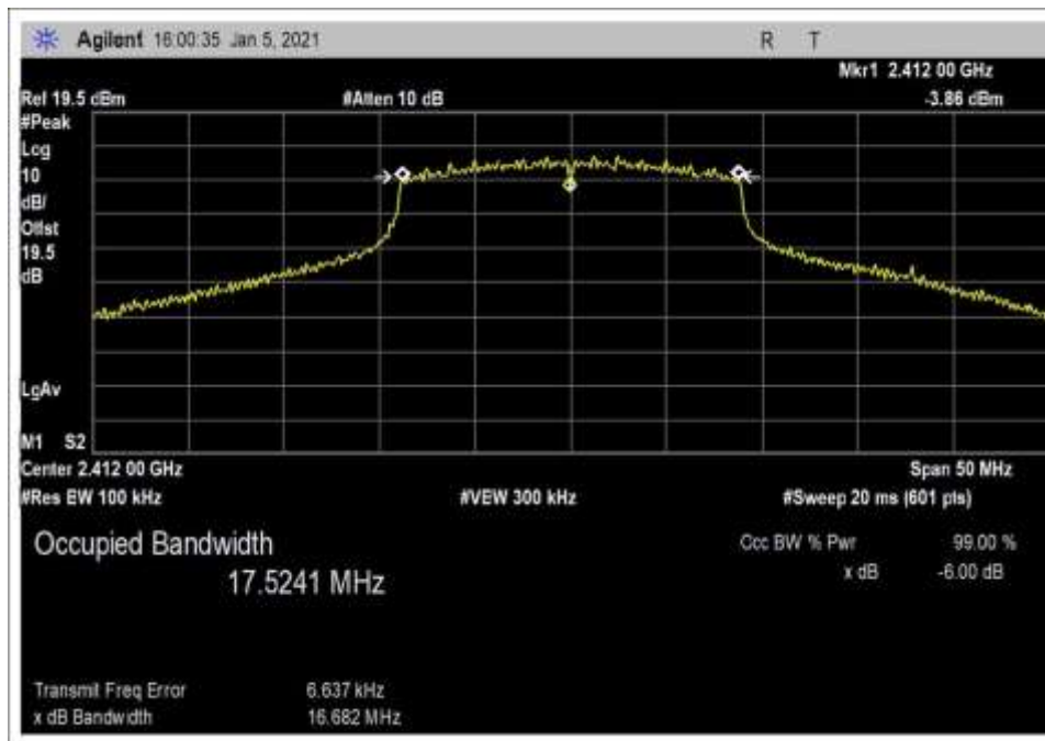
-6dB_BW_802.11n_Low Channel_17dBm
