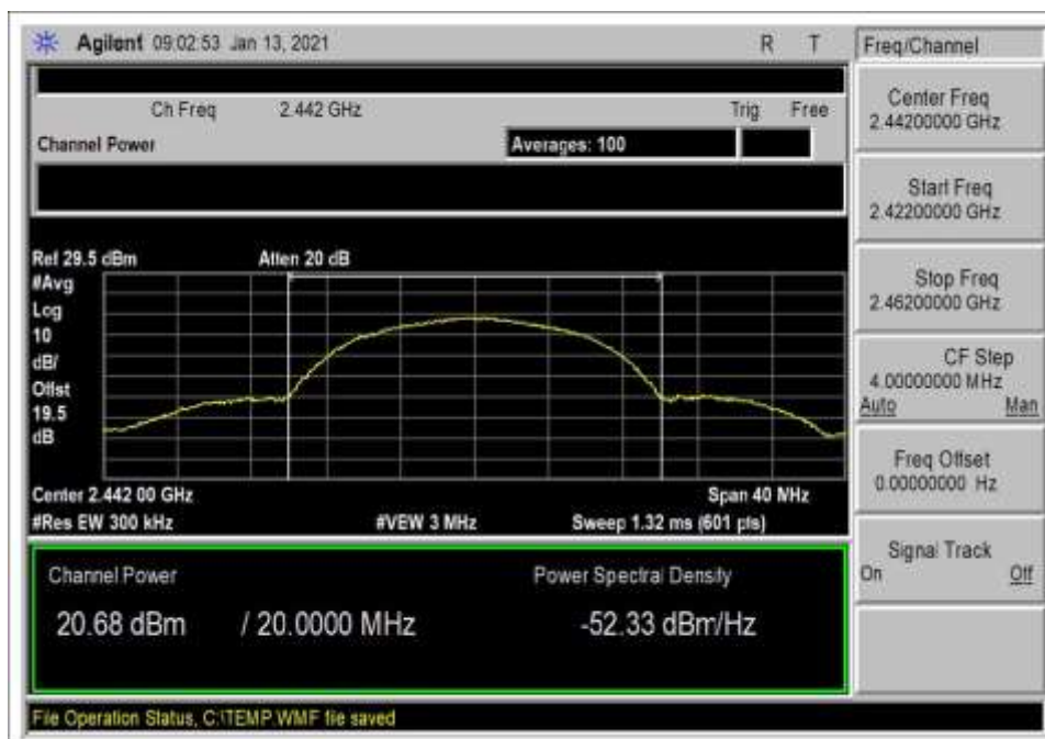
power_802.11b_Middle Channel_19dBm
