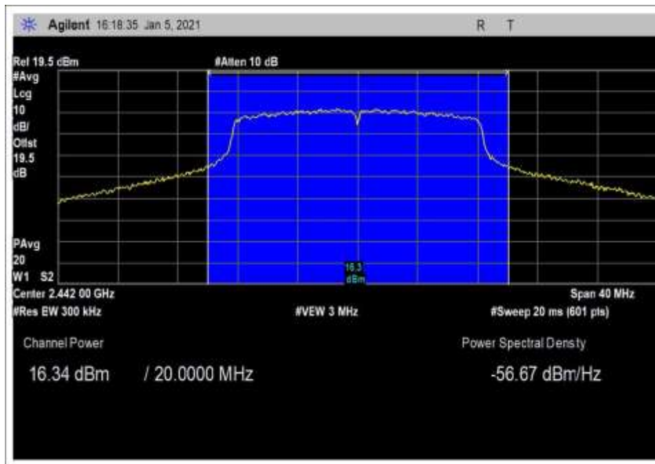
power_802.11g_Middle Channel_17dBm
