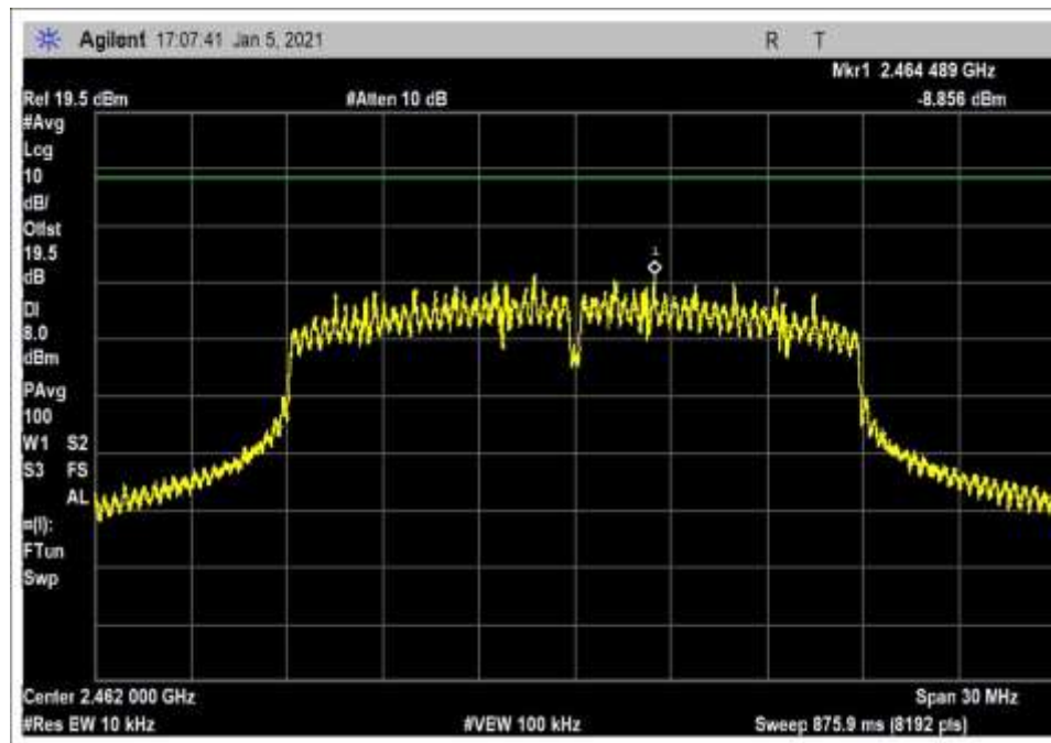
PSD_802.11n_High Channel_17dBm
