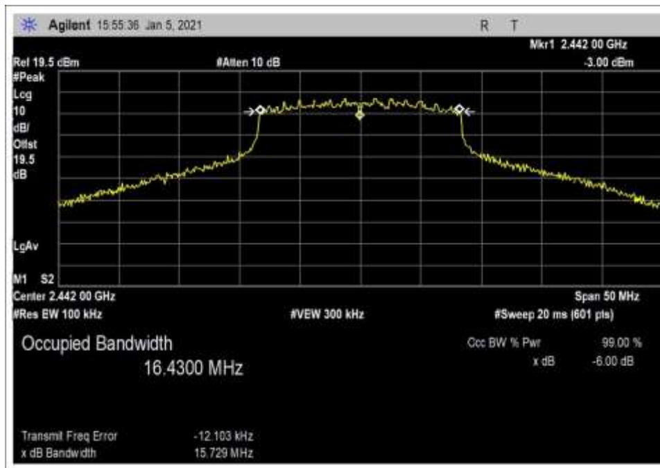
-6dB_BW_802.11g_Middle Channel_17dBm
