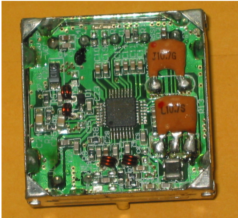
Picture of UHF module of HP1392
