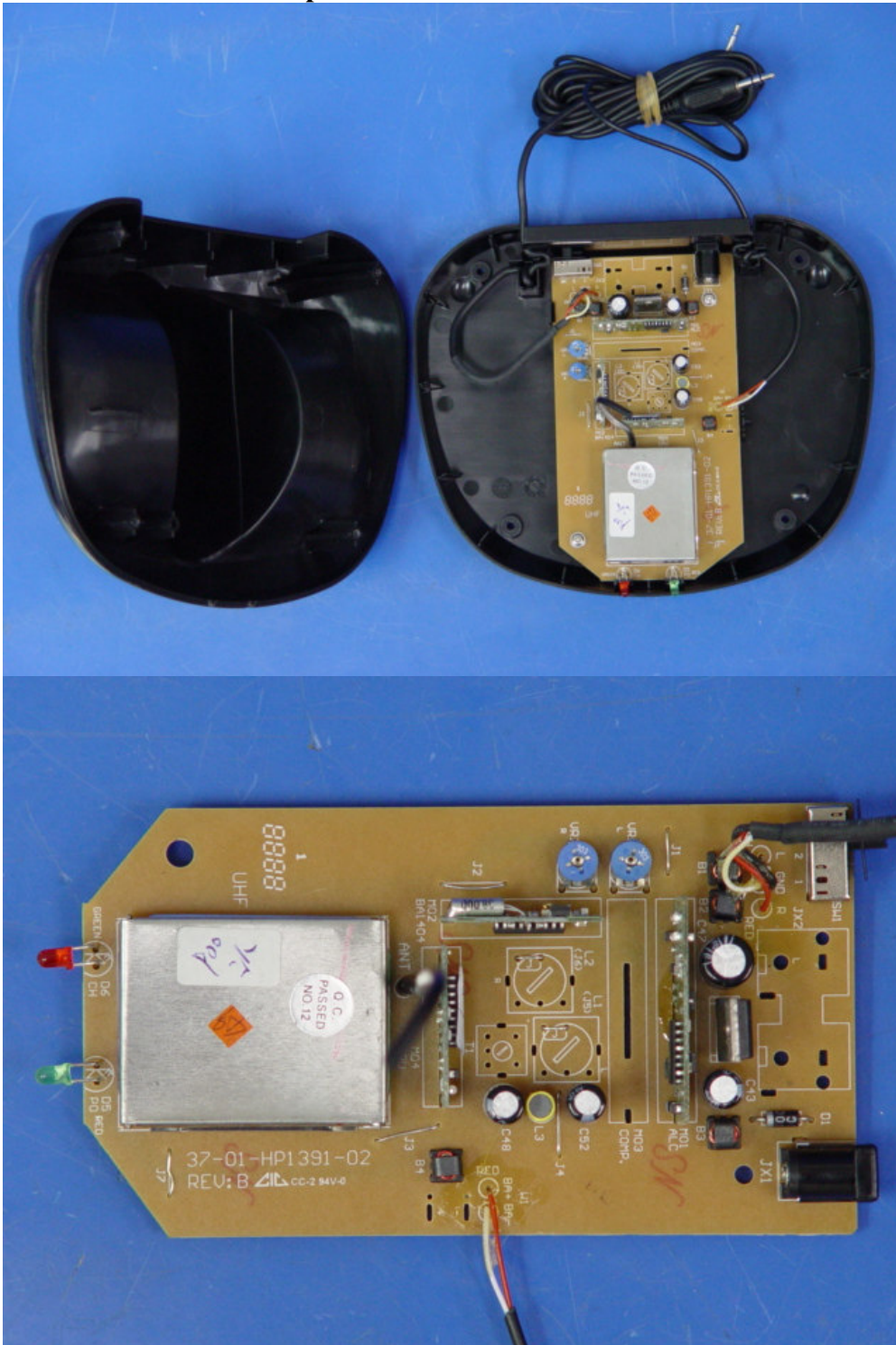
HP1391 and HP1491 internal photo
