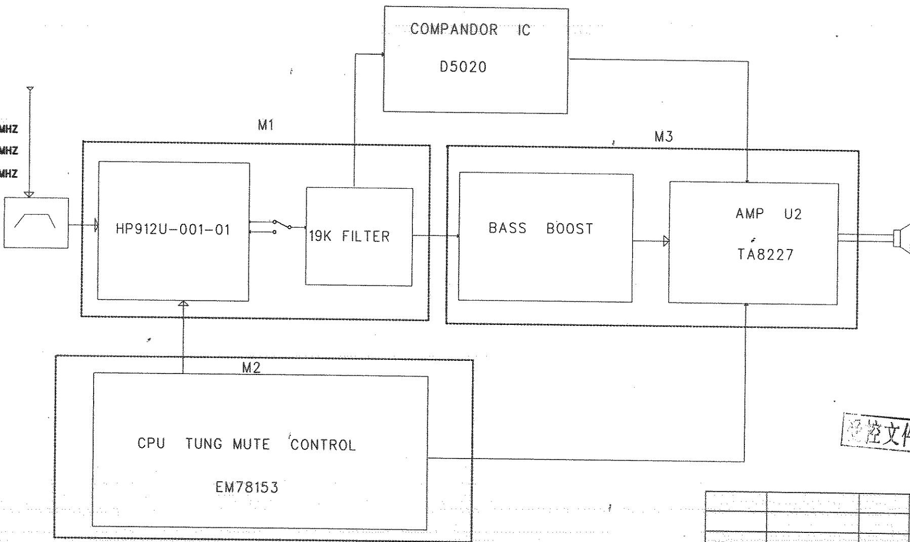
BLOCK DIAGRAM OF SP1552
