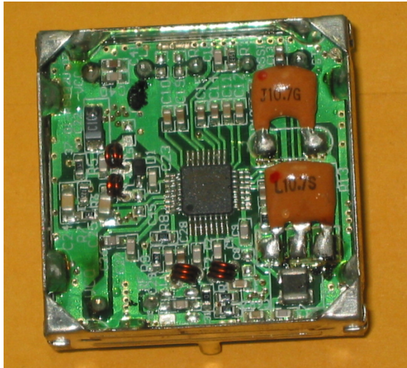
Picture of UHF module of HP1552
