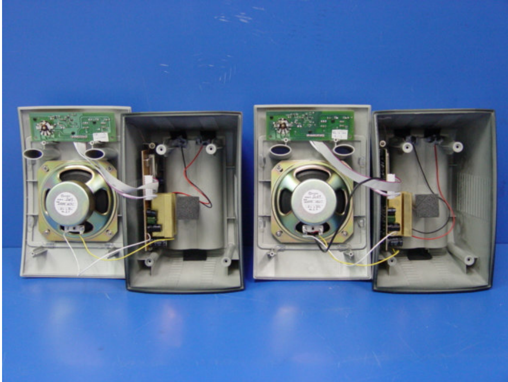
Internal Picture of HP1552
