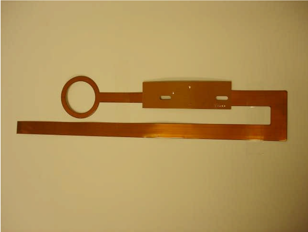
RFID board and antenna - solder side
