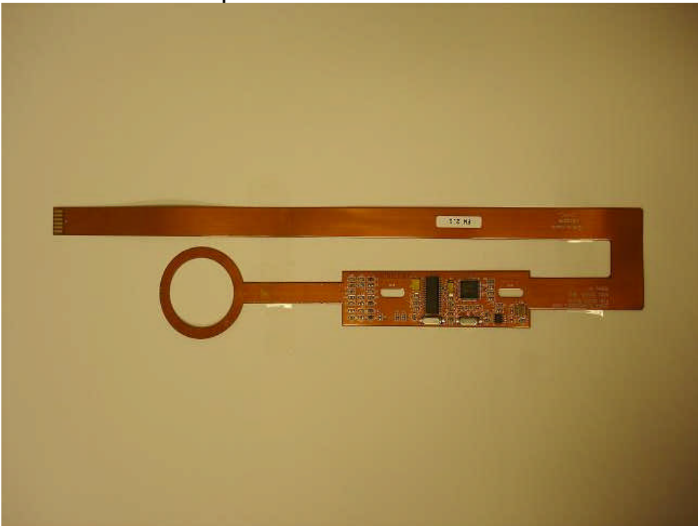
RFID board and antenna - component side
