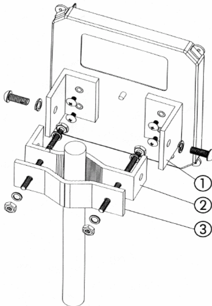
Figure 5 – Assembling the Mounting Kit to the P-780
