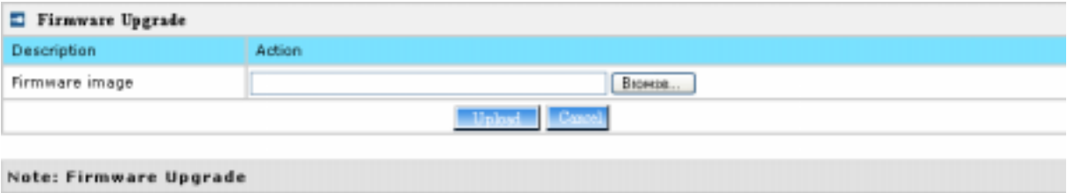
Figure 63 – Firmware Upgrade
