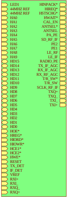
WL-373-2 WL-375S2V02A.SCH
