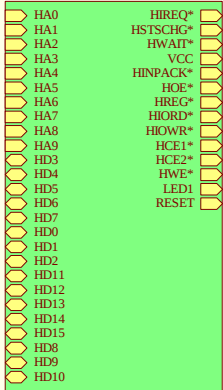
WL-373-1 WL-375S1V02A.SCH
