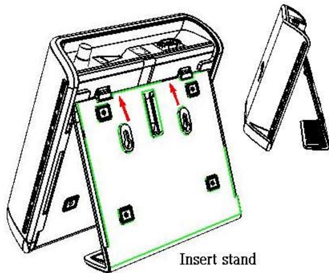
figure 6 – insert stand
