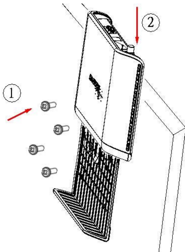
figure 7 — wall mount
