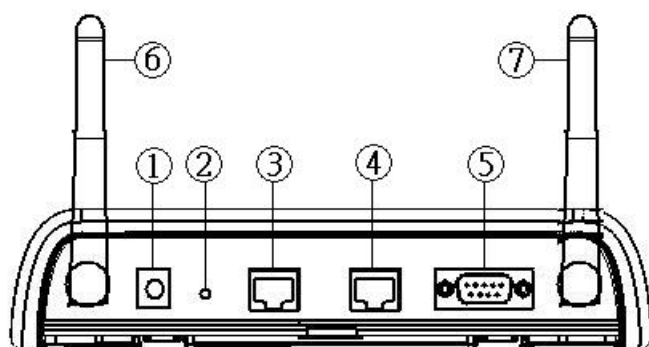
Figure 4 – Connectors
