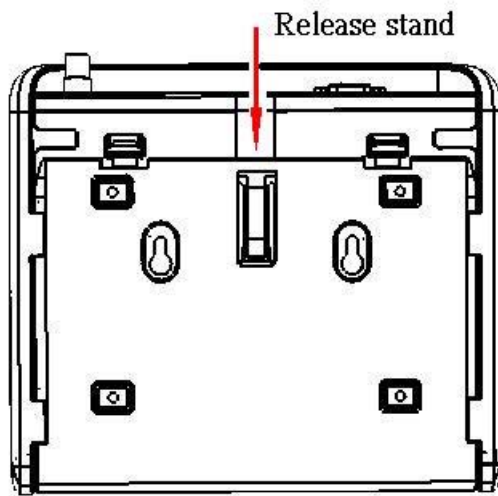
figure 5 – release stand
