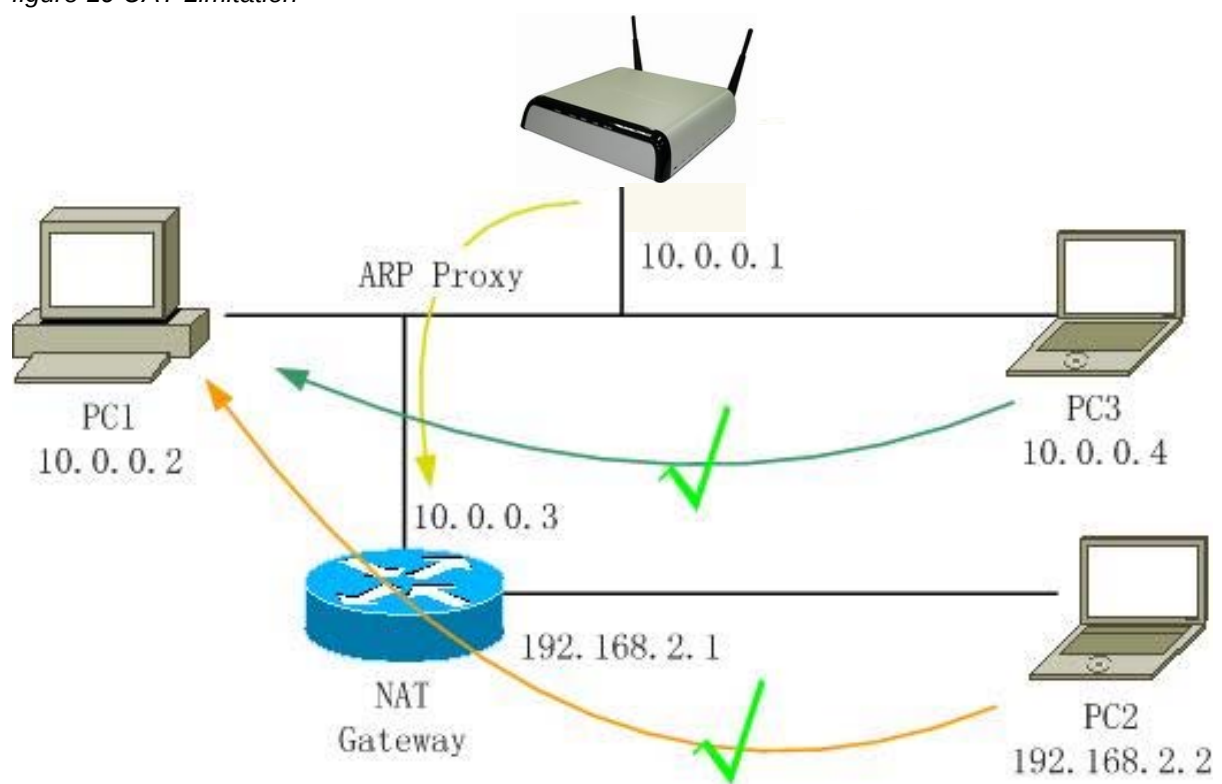
figure 19 UAT Limitation
