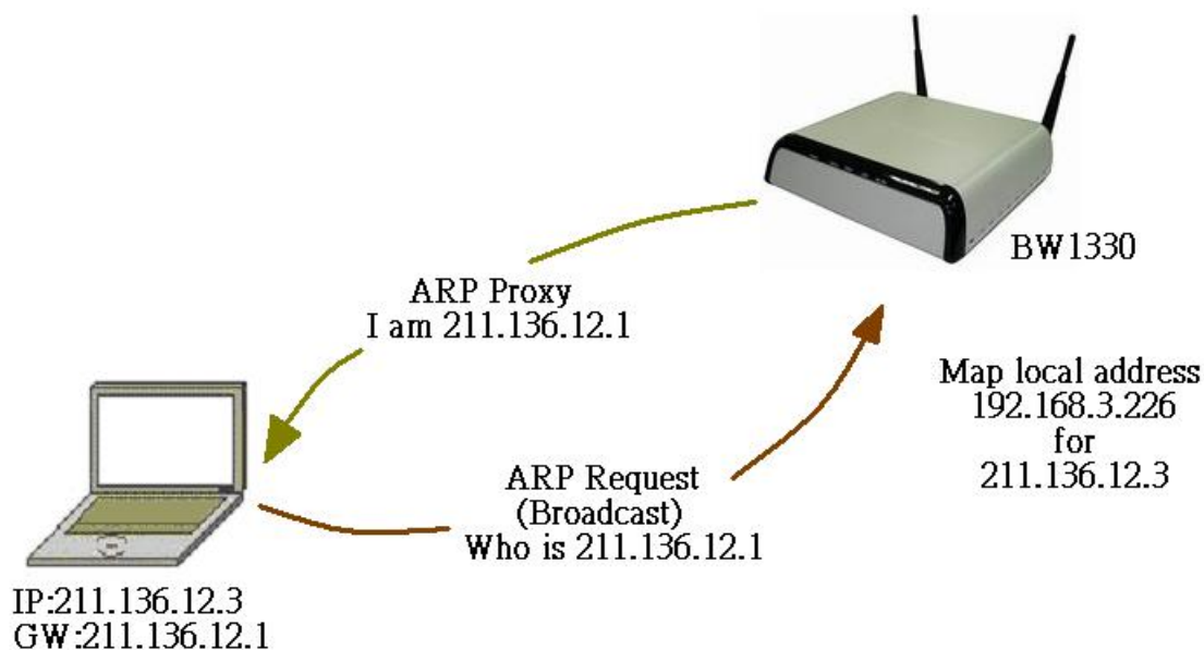
Figure 18 – UAT Principle
