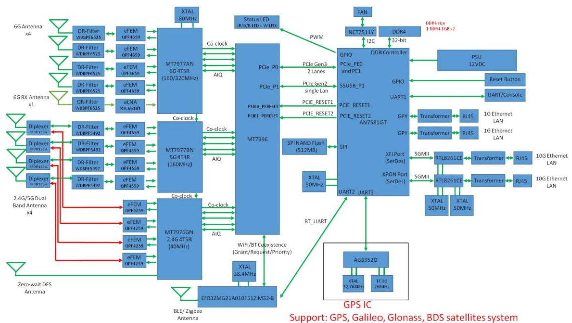
Figure 1. Function Block Diagram of the W1700 AP
