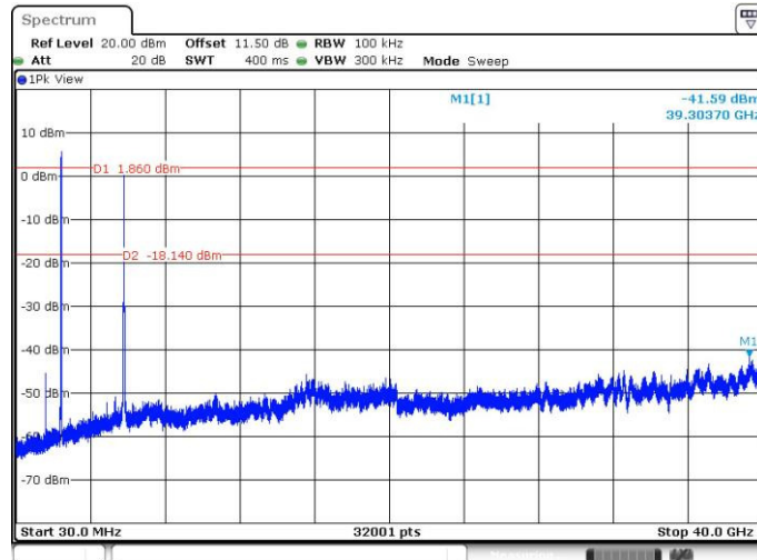
Conducted Emission Plot of Antenna port 1
