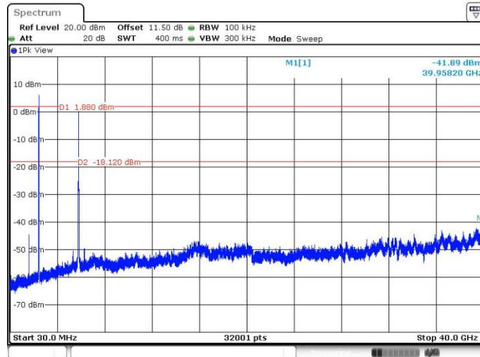
Conducted Emission Plot of Antenna port 0
