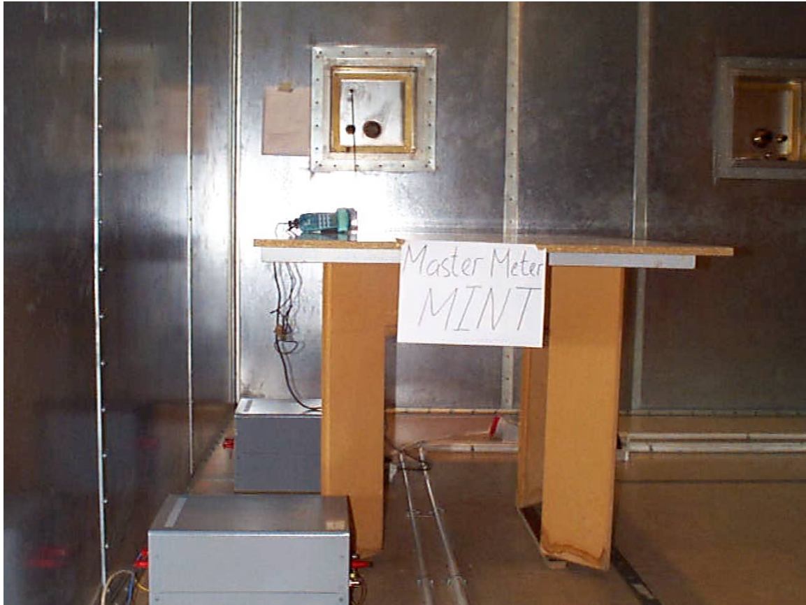
Figure 2 Conducted Emission Test. Side
