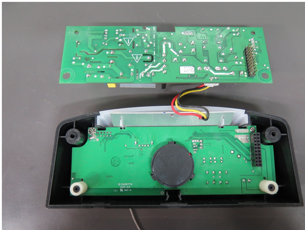
MQ-800 POWER BOARD AND MAIN BOARD
