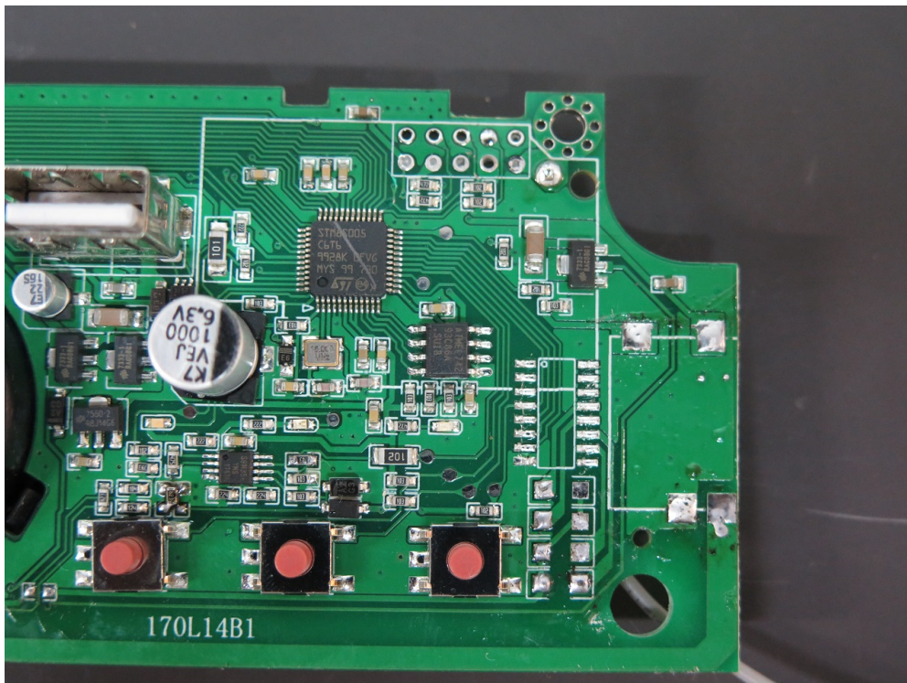
MQ-800 PCB BELOW TX AND RX MODULE
