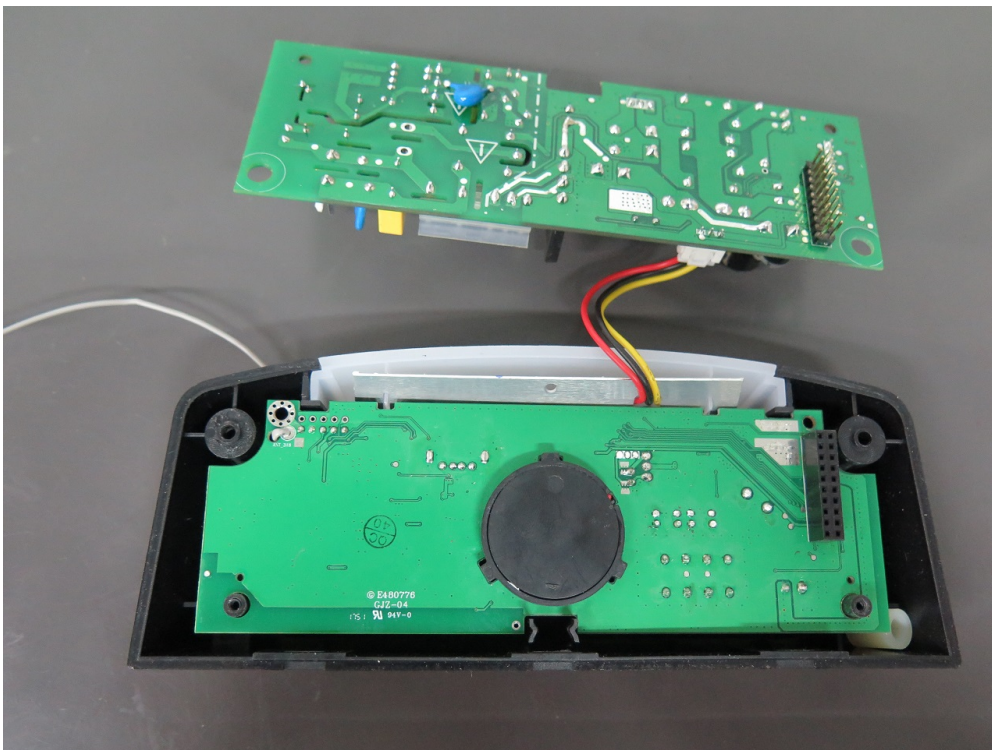
LQ-803 POWER BOARD AND MAIN BOARD
