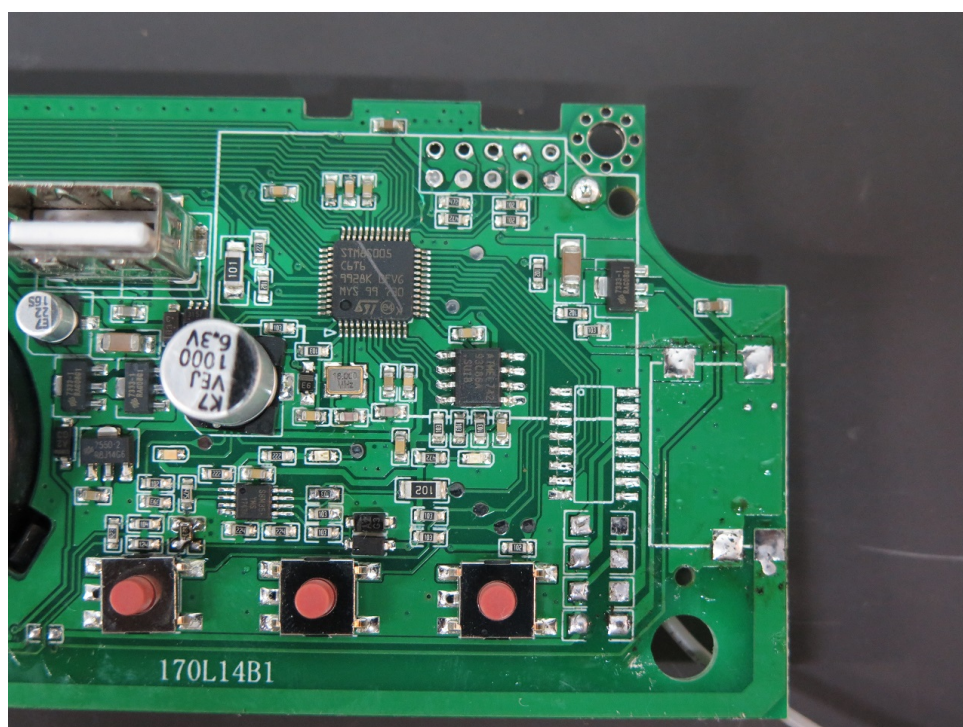
LQ-803 PCB COVERED BY TX ND RX MODULE
