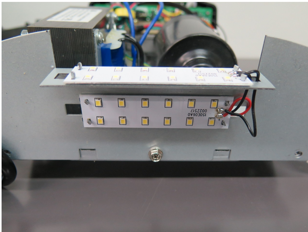
LQ-803 BACK LEDD BOARDS
