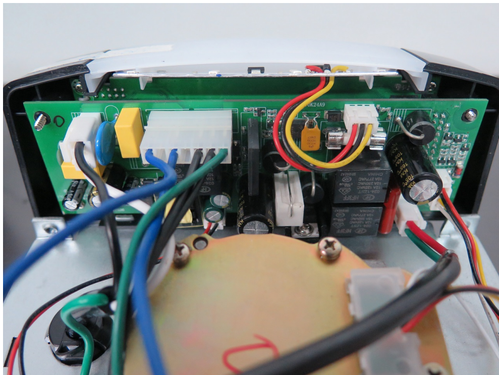
LQ-803 POWER BOARD WIRING
