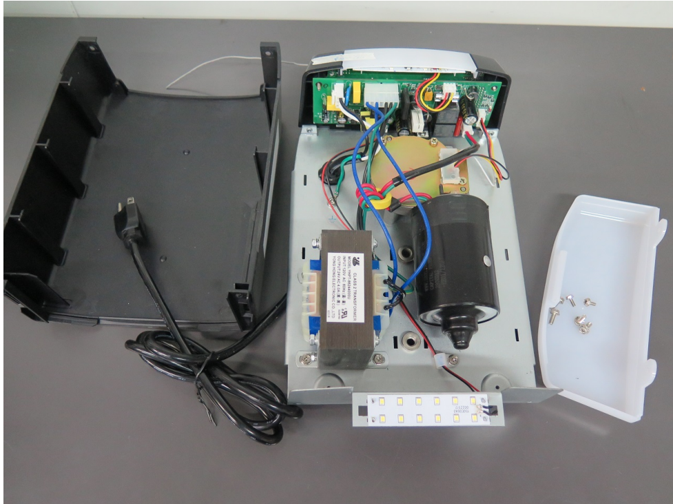
LQ-803 INTERNAL CONSTRUCTION
