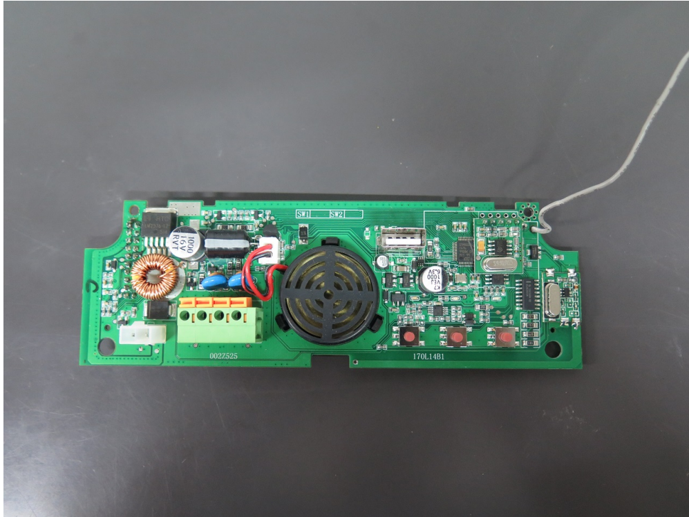
LQ-803 MAIN BOARD
