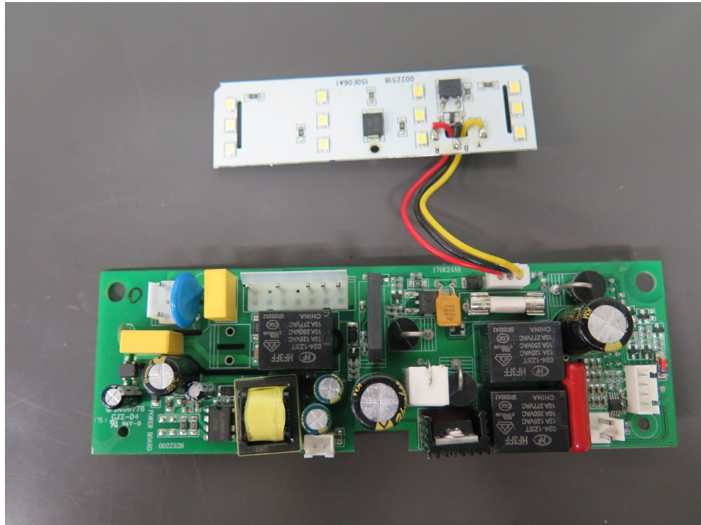
LQ-803 POWER BOARD AND FRONT LED BOARD
