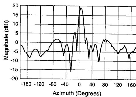
Horizontal Pattern (dB)
