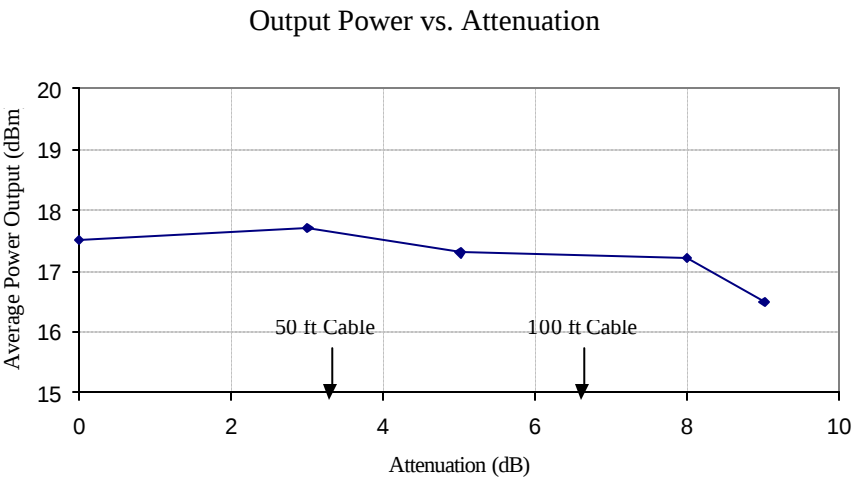
Figure 2. Plot of Output Power vs. Input Signal Attenuation
