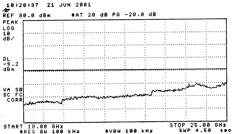
Figure 6.5 Antenna conducted spurious emissions, high channel.
