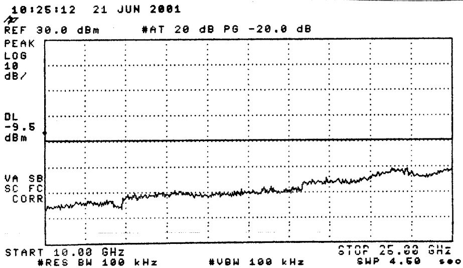
Figure 6.4 Antenna conducted spurious emissions, mid channel.
