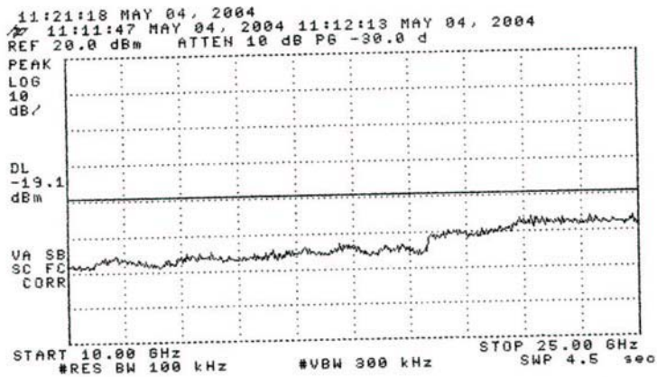
Figure 6.2. Spurious Emissions – 16.0 dBm Amp: CH: 2437
