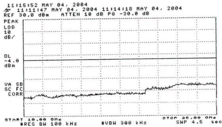
Figure 6.3. Spurious Emissions – 29.6 dBm Amp: CH: 2437
