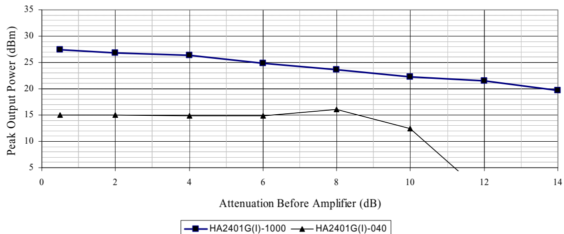
Figure 4.1. Peak Amplifier Output Power vs. Cable Attenuation
