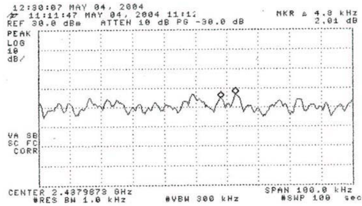
Figure 6.13. Power Spectral Density – 29.6 dBm Amp: CH: 2437
