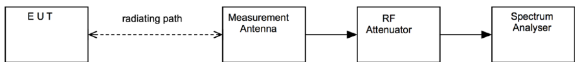
Figure viii Test Setup
