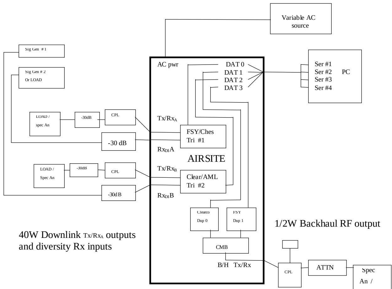
Figure 14A - (AdaptaSite) 1B Test Configuration Intermodulation Distortion Setup
