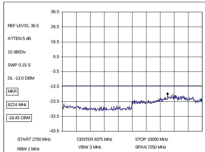
Figure 3.4.3: Conducted Spurious, Downlink, 2.75 to 10 GHz
