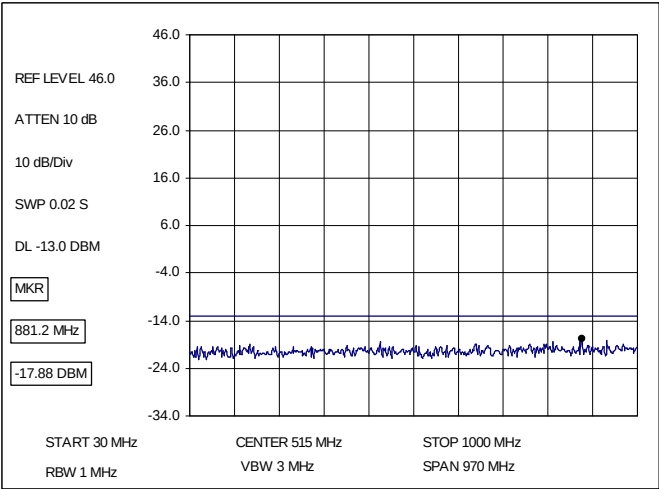
Figure 3.4.1: Conducted Spurious, Downlink, 30 to 1000 MHz
