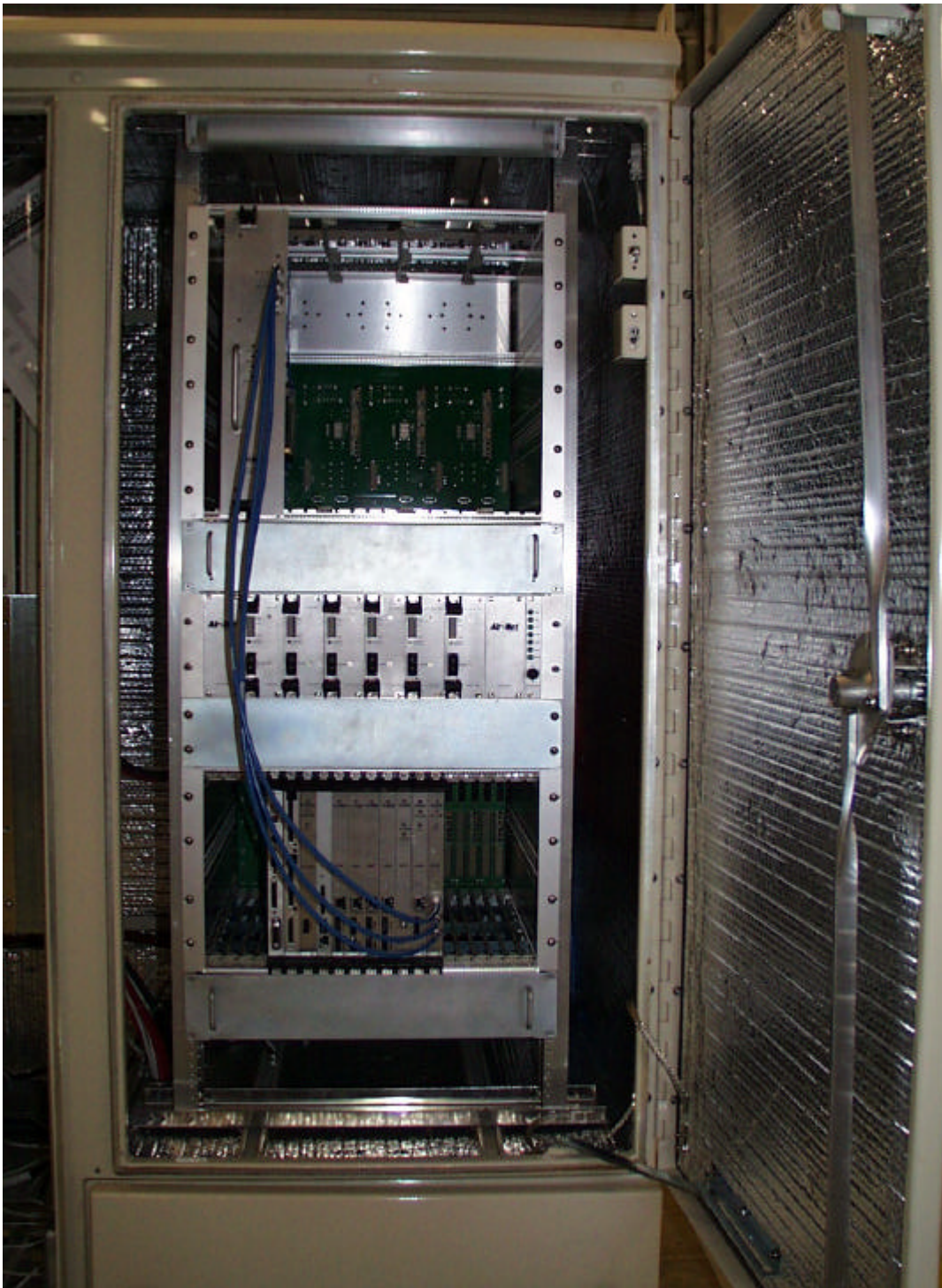
Photograph 3: Outdoor Enclosure – Front view door open, right side
