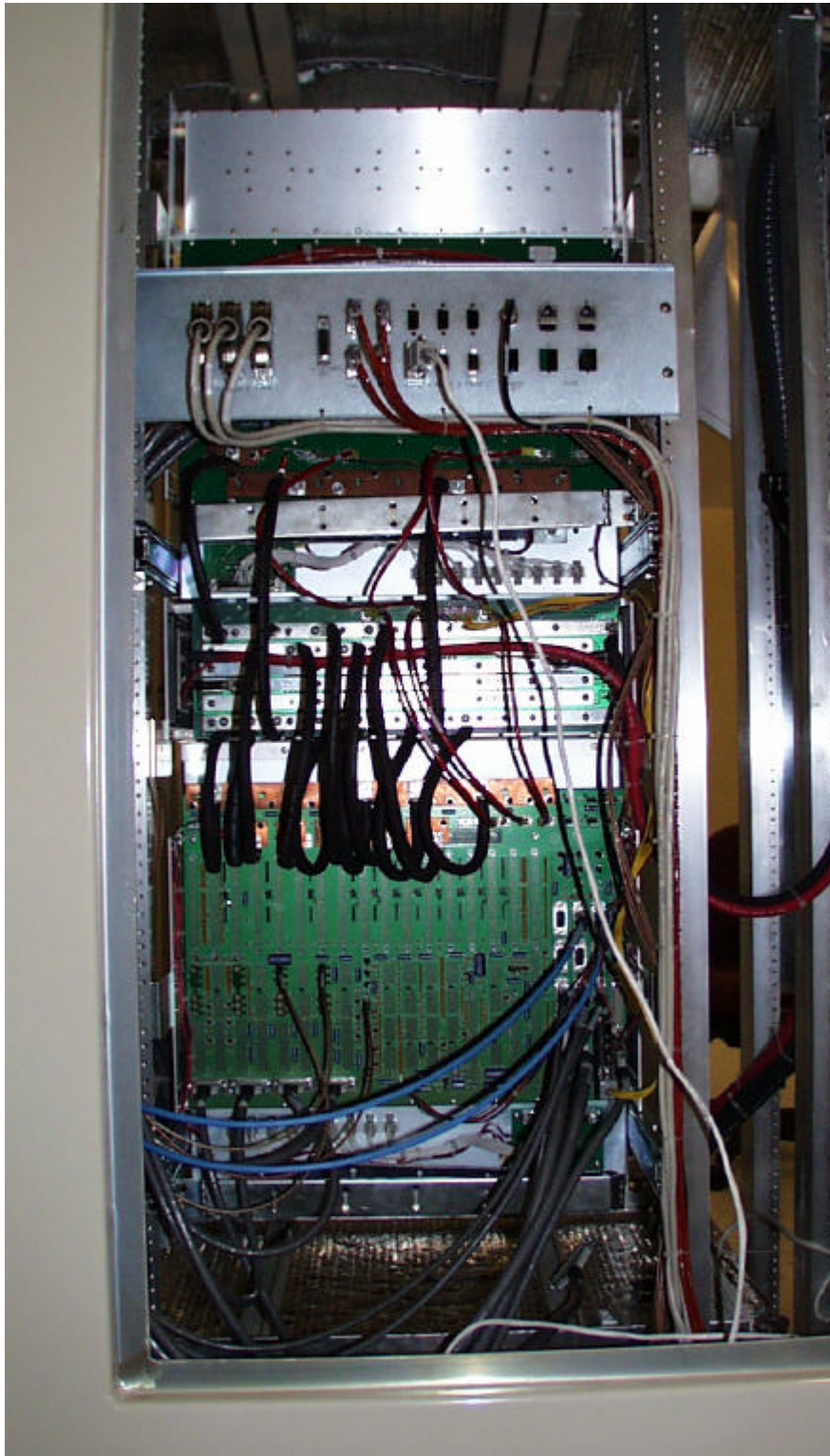
Photograph 7: Outdoor Enclosure – Rear view door open, Left side
