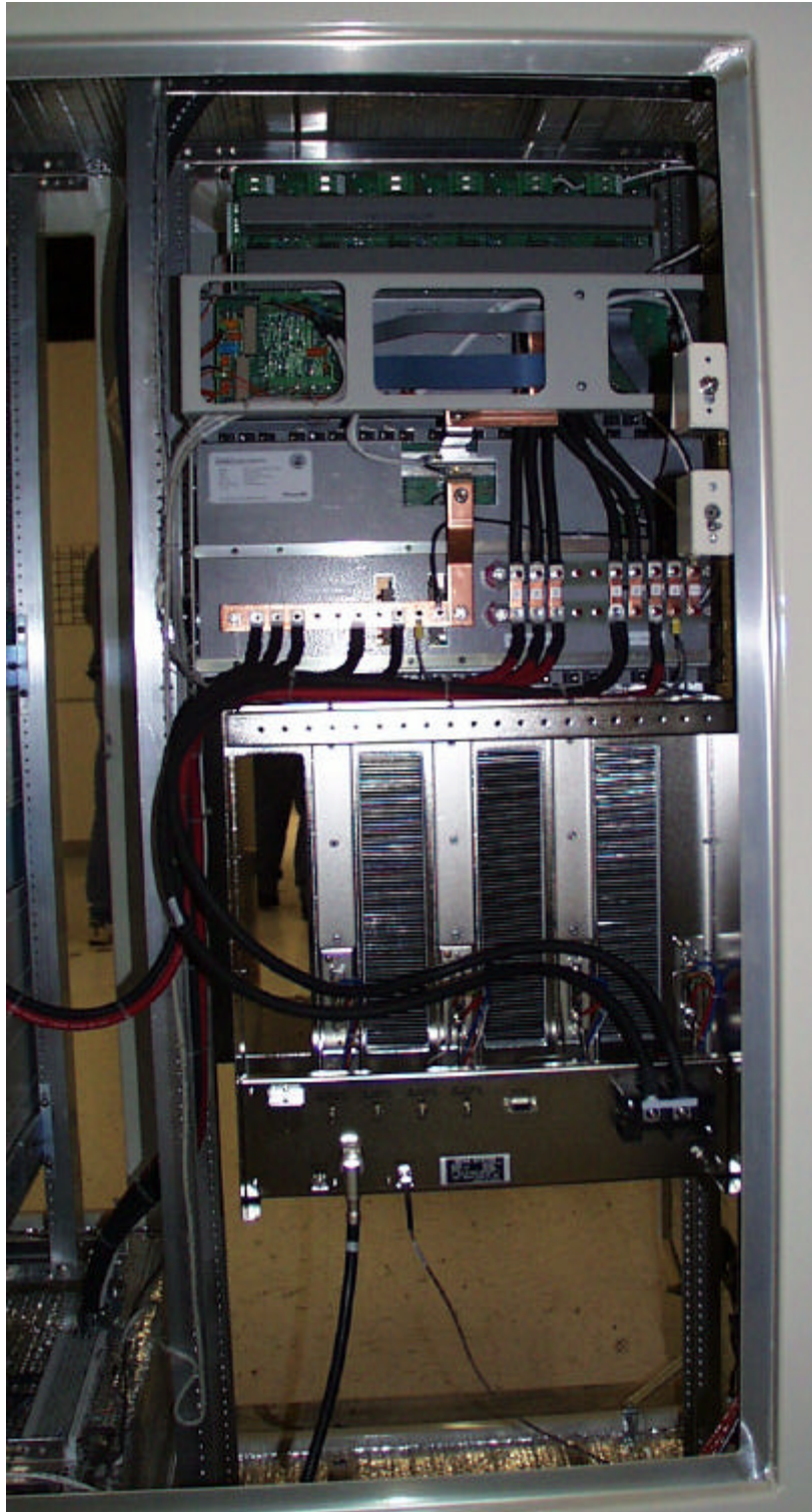
Photograph 6: Outdoor Enclosure – Rear view door open, Right side
