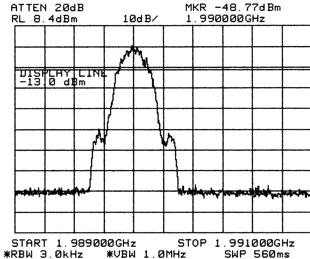
Figure 7.3.2: Upper Band Edge Plot
