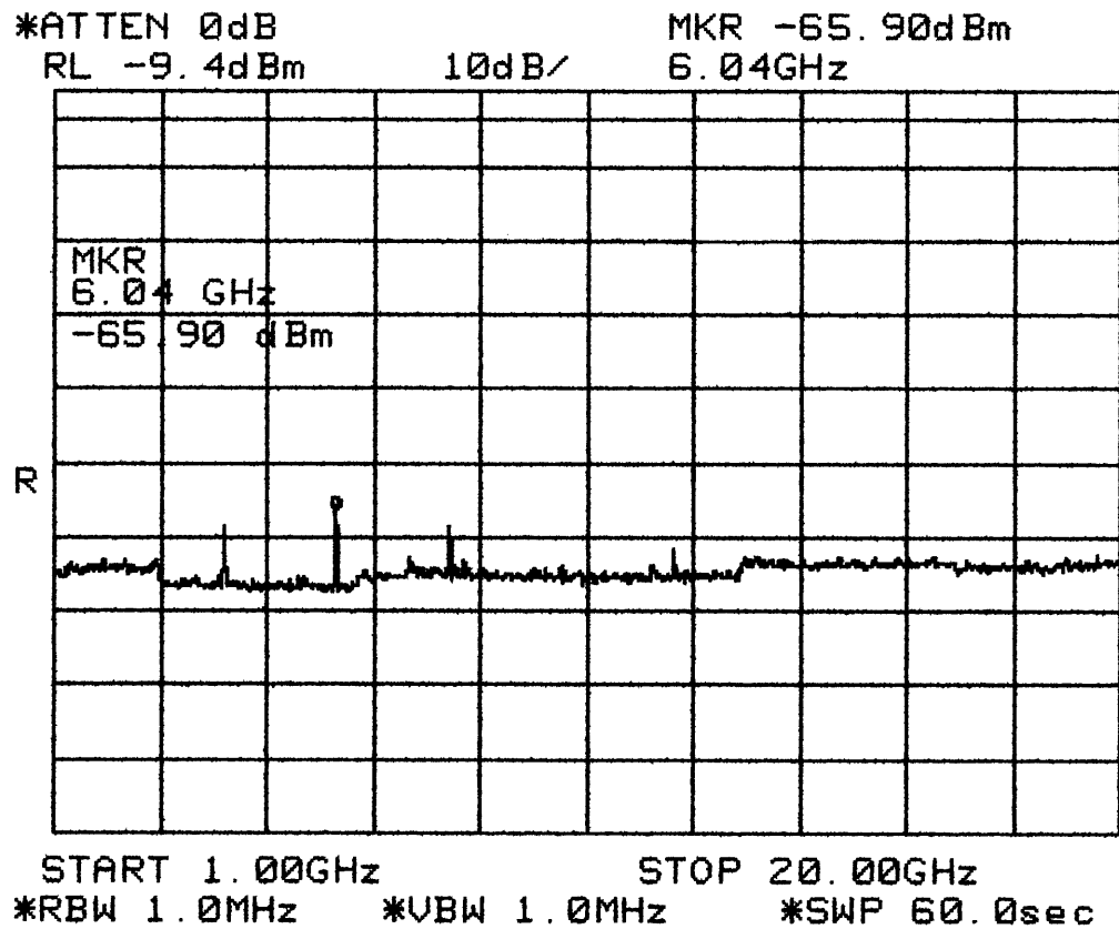
Figure 7.4.6: Conducted Spurious, Receive Port B, 1 to 20 GHz
