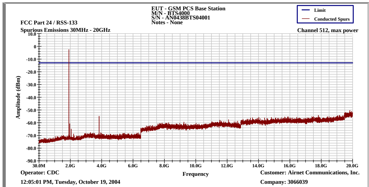
Figure 5-1: Out of band emissions at antenna terminals, Channel 512
