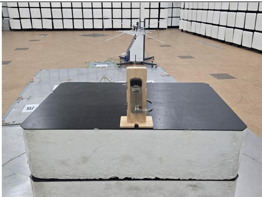
[Rear view of Radiated Emission (Below 1GHz)]_ YMC654-4(Alt. Model)
