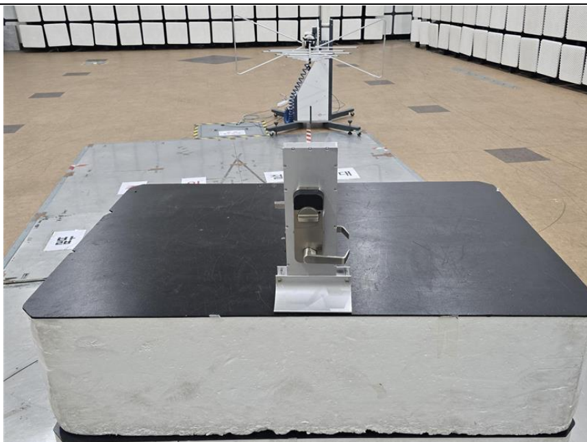
[Rear view of Radiated Emission (Below 1GHz)]_ YMC614-5.5(Alt. Model)
