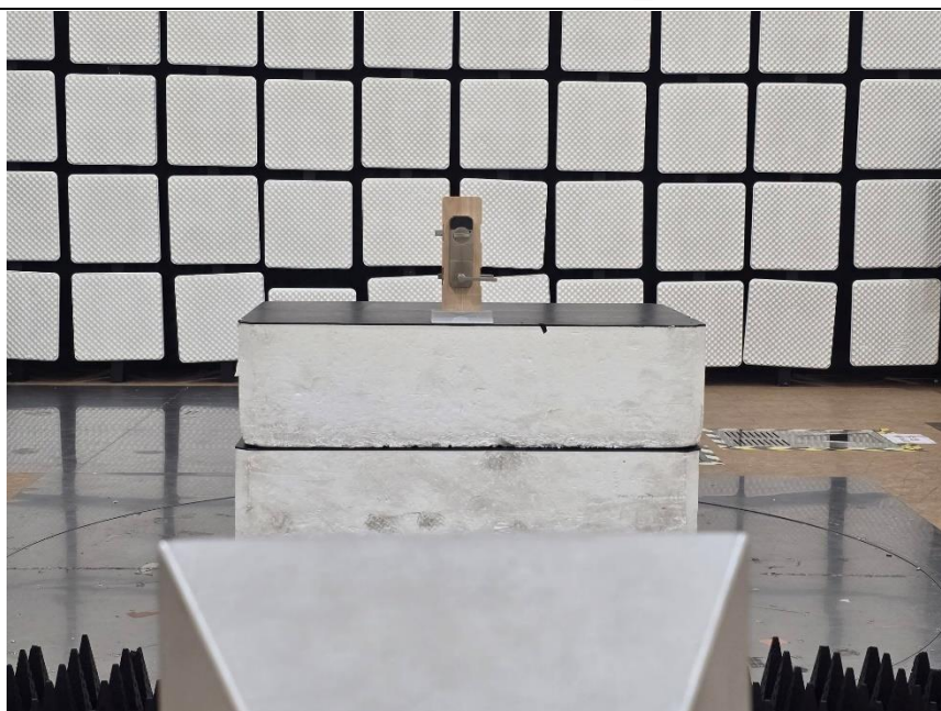
[Rear view of Radiated Emission (Above 1GHz)]_ YMC634-4(Alt. Model)
