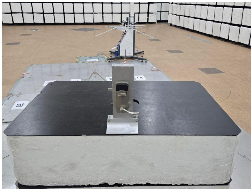
[Rear view of Radiated Emission (Below 1GHz)]_ YMC624-5.5(Basic Model)
