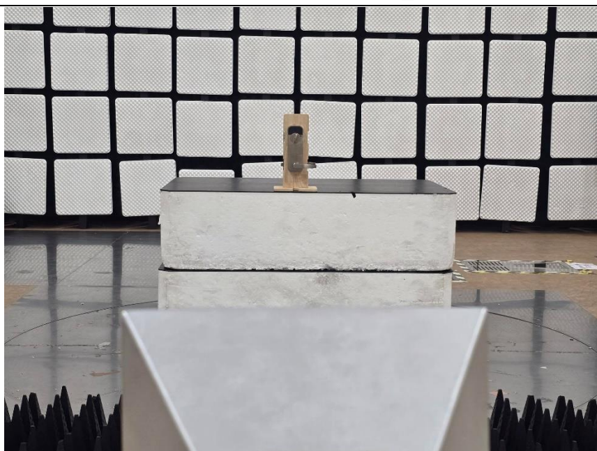
[Rear view of Radiated Emission (Above 1GHz)]_ YMC654-4(Alt. Model)
