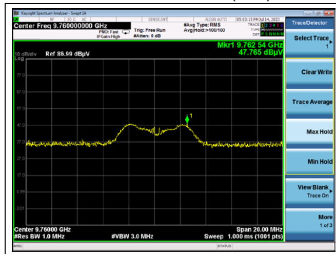
Channel 18 4 th Harmonic (Peak)
