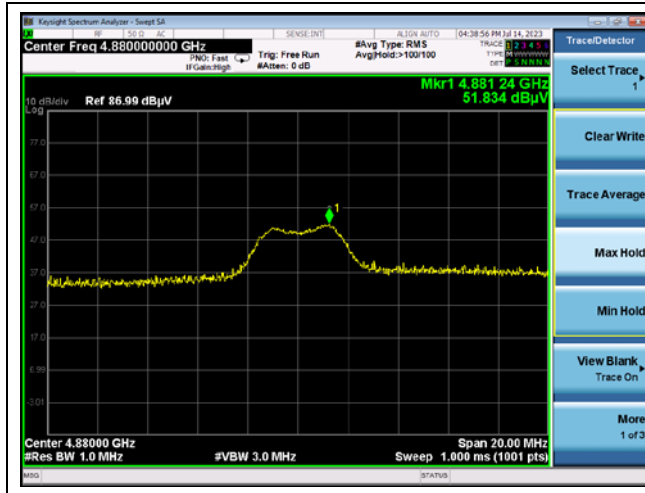
Channel 18 2 nd Harmonic (Peak)
