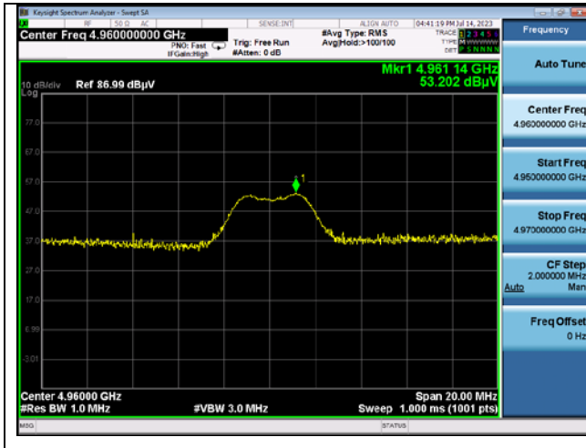
Channel 26 2 nd Harmonic (Peak)
