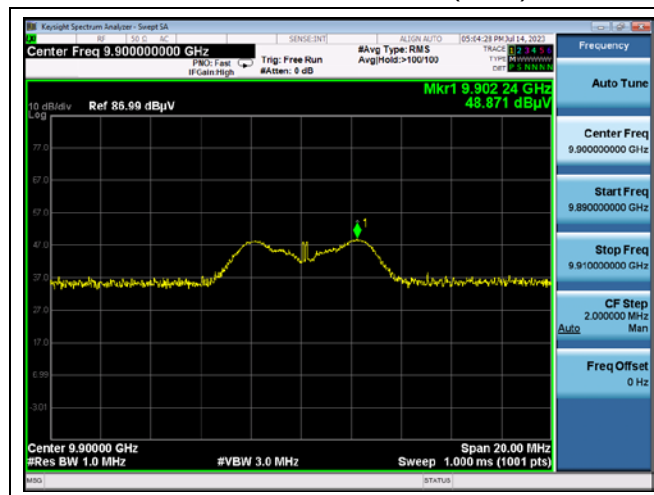
Channel 25 4 th Harmonic (Peak)
