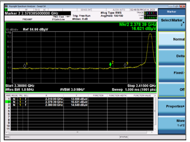
Channel 12 band edge (Average)
