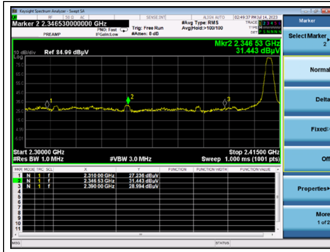
Channel 12 band edge (Peak)
