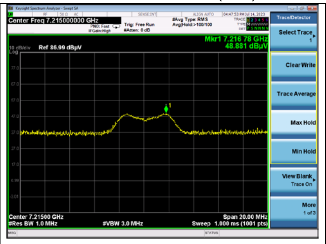
Channel 11 3 rd Harmonic (Peak)
