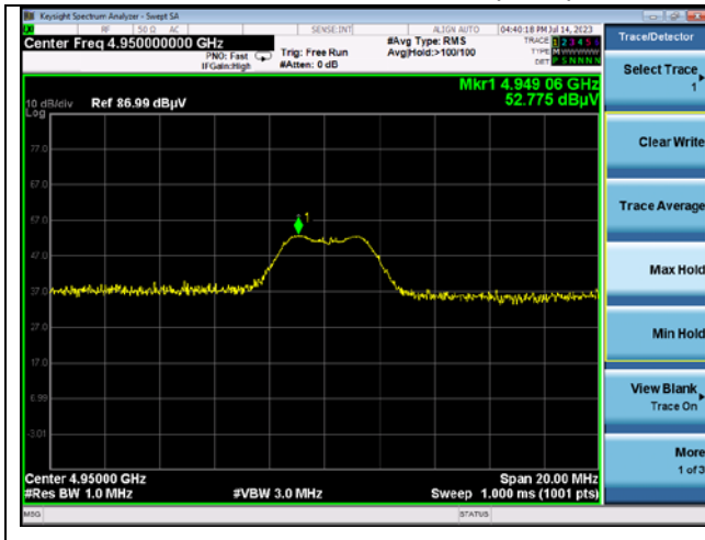
Channel 25 2 nd Harmonic (Peak)
