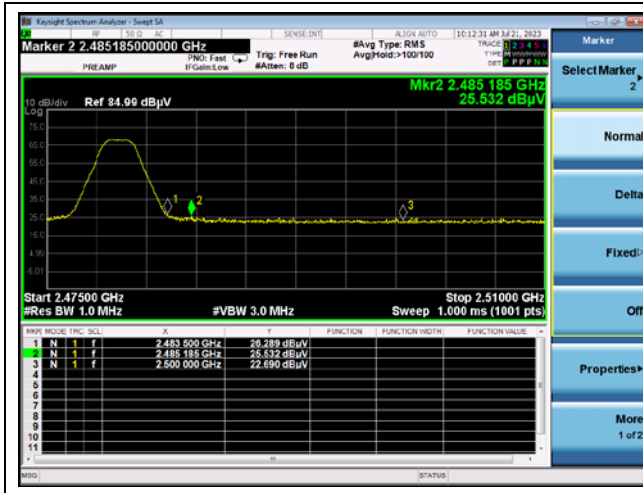
Channel 26 band edge (Peak)
