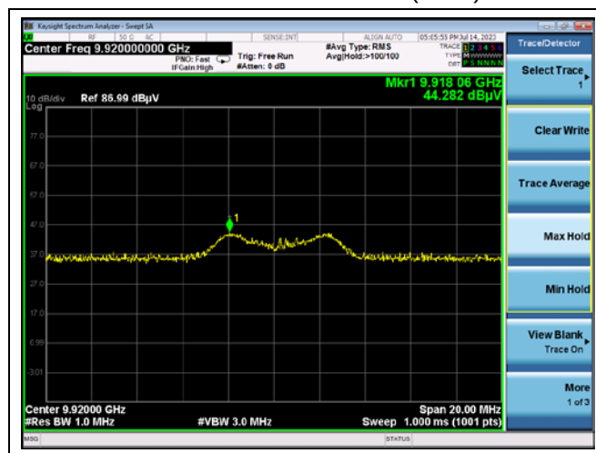
Channel 26 4 th Harmonic (Peak)
