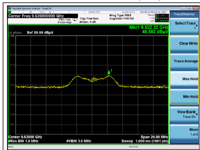
Channel 11 4 th Harmonic (Peak)
