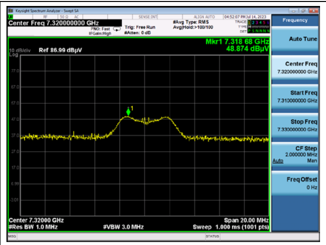
Channel 18 3 rd Harmonic (Peak)
