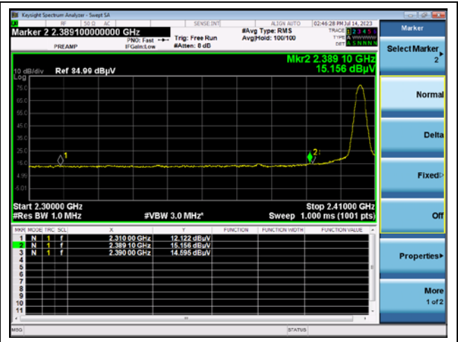
Channel 11 band edge (Average)
