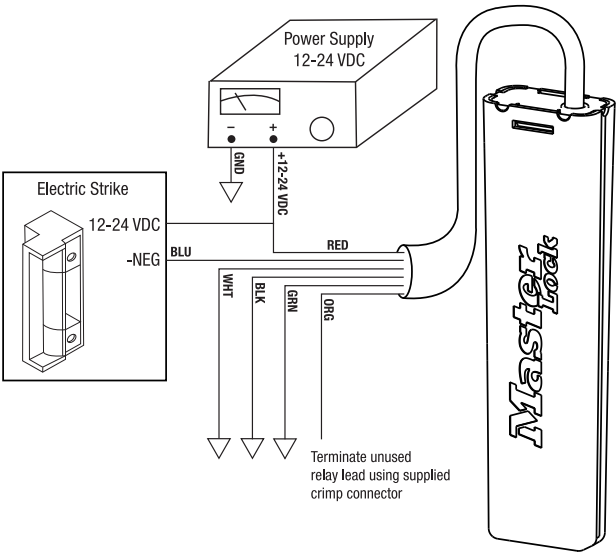
Diagram 1: Wiring for Electric Strike
