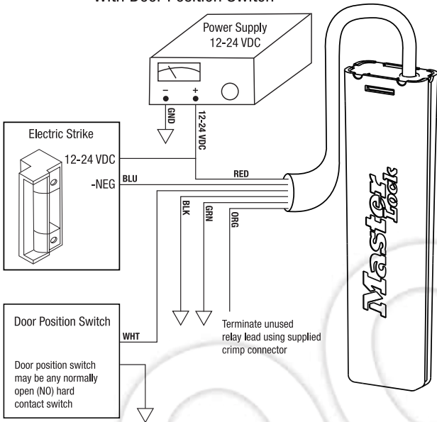
Diagram 2: Wiring for Electric Strike With Door Position Switch
