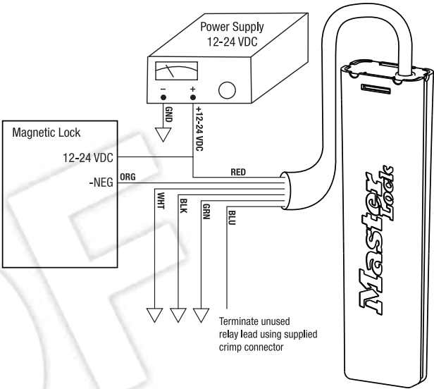
Diagram 3: Wiring for Magnetic Lock
