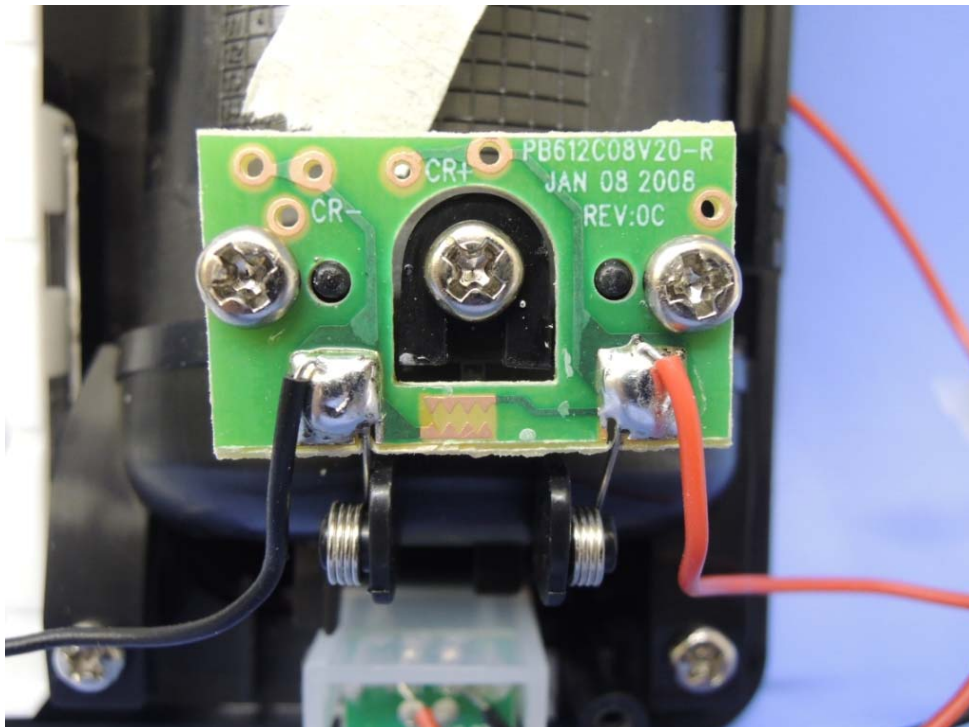
Base Unit - Charge contact PCB solder side
