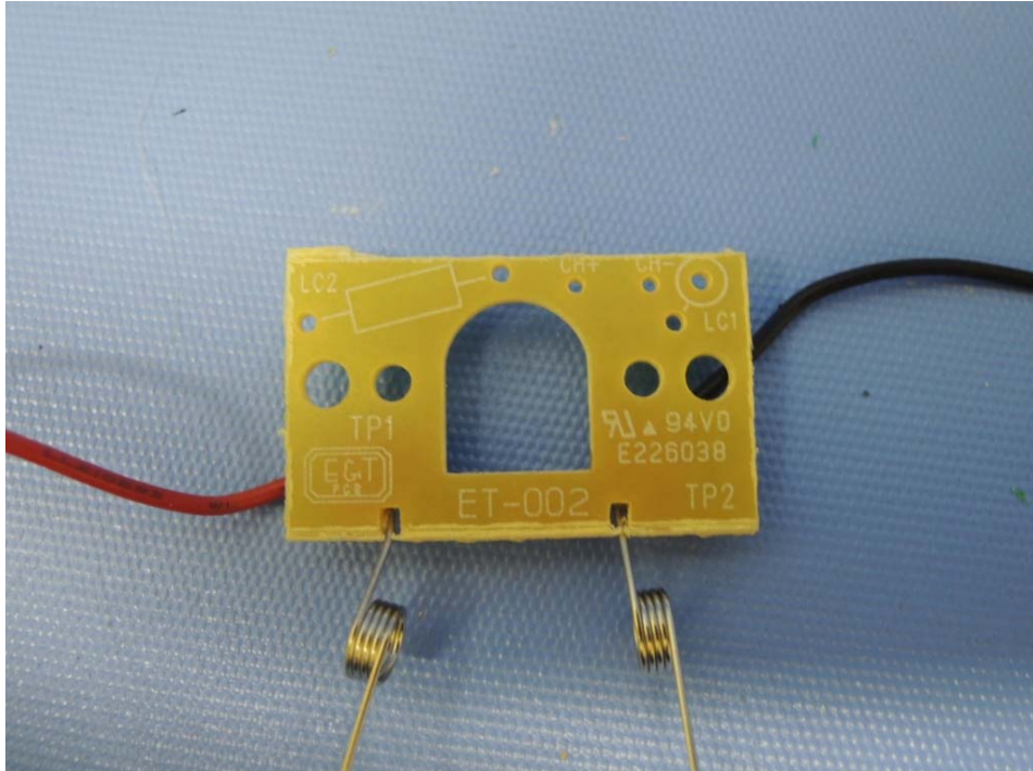
Base Unit - Charge contact PCB comp side
