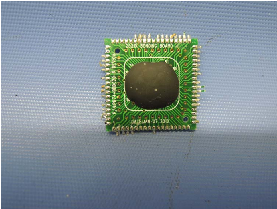
Base Unit MCU PCB comp side
