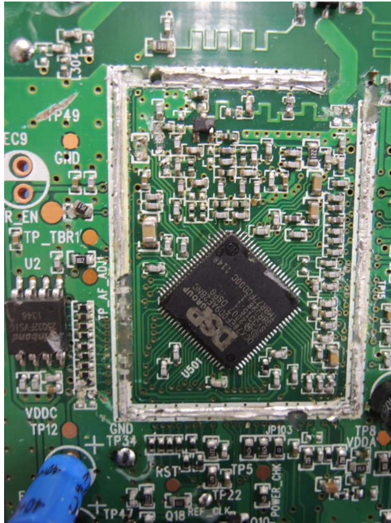
Base Unit Oscillator comp side
