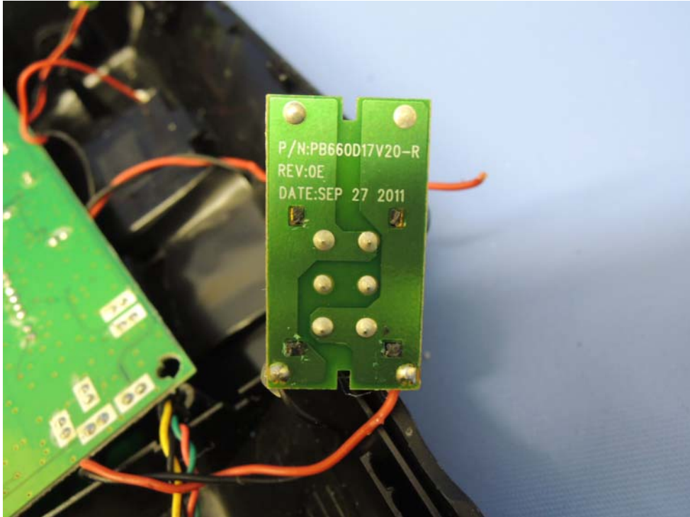
Base Unit Hookswitch PCB solder side
