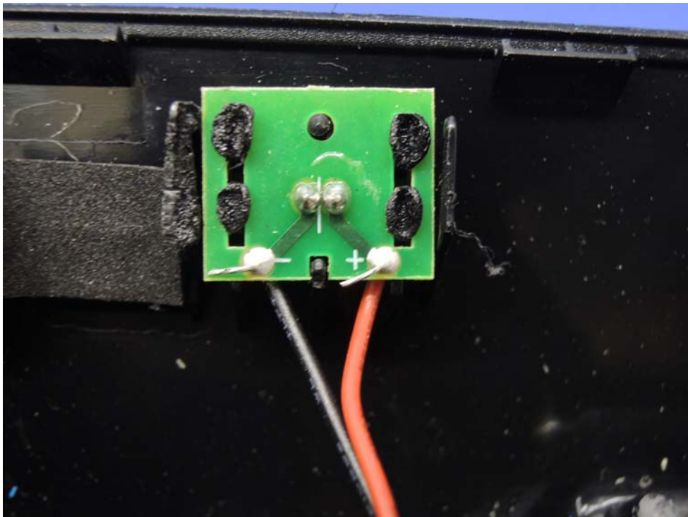
Base Unit Mic PCB solder side
