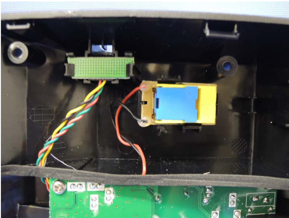
Base Unit Hookswitch PCB comp side
