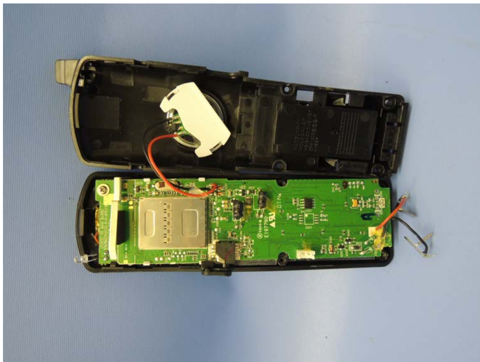
Handset assembly
