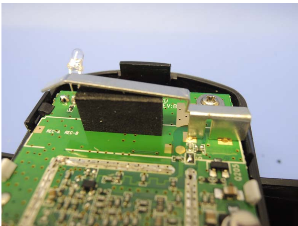
Handset Antenna
