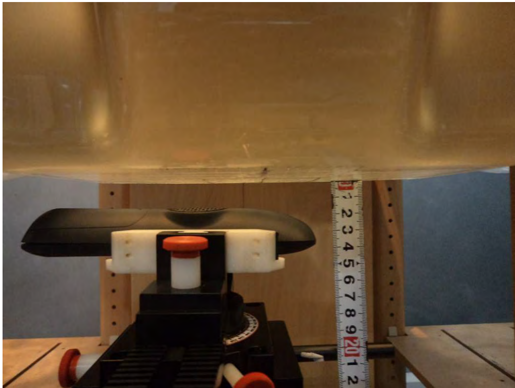
Body-Back-Headset Setup Photo (15mm)
