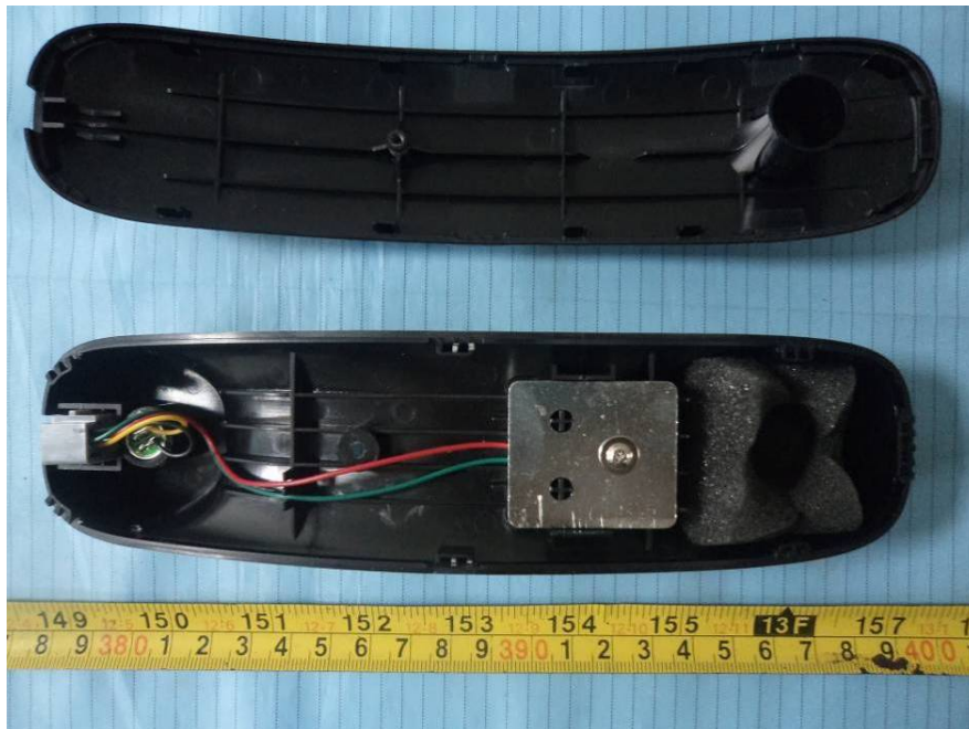
EUT – Handset Cover off View
