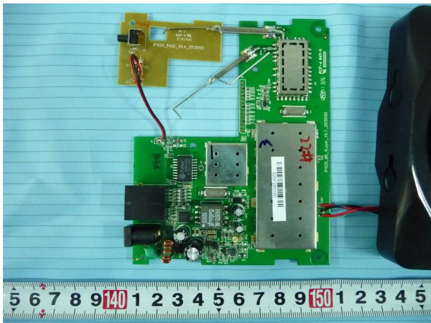
EUT – Main Board Top View (Base)
