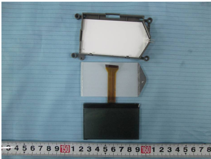
EUT – LCD Screen Cover off View
