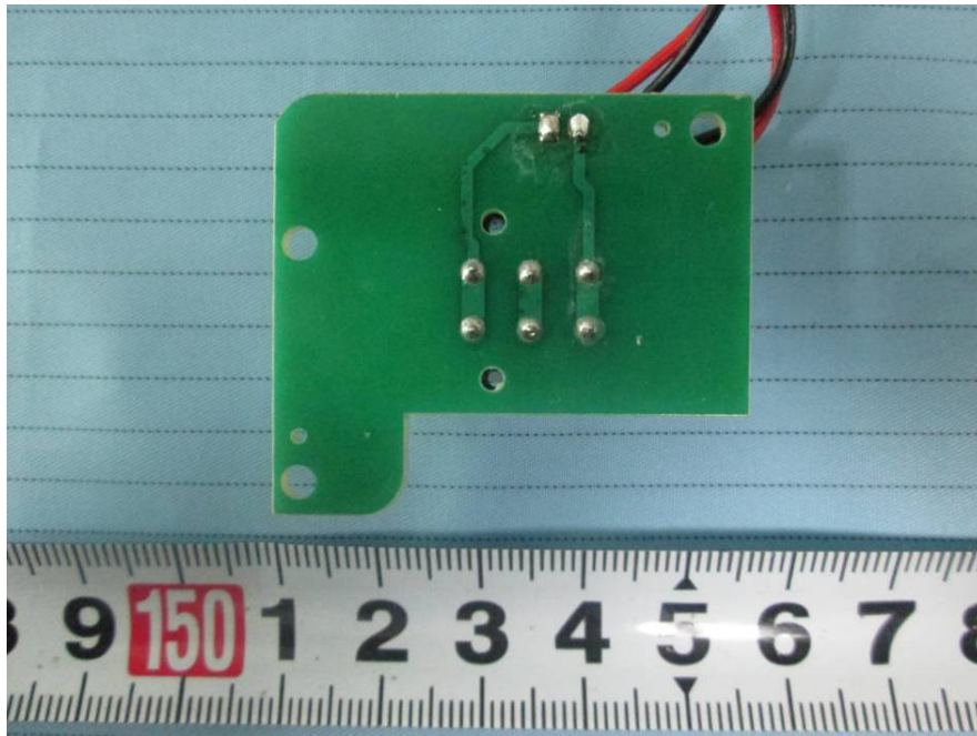
EUT – HOOK PCB Bottom View
