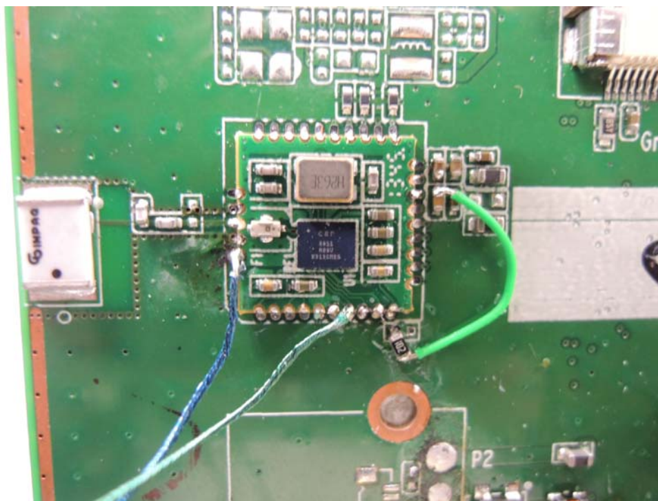
Base Unit Bluetooth RFIC and Antenna
