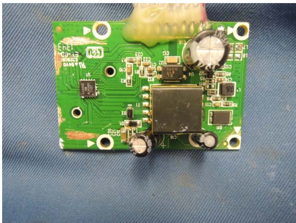
Base Unit PCB2 component side
