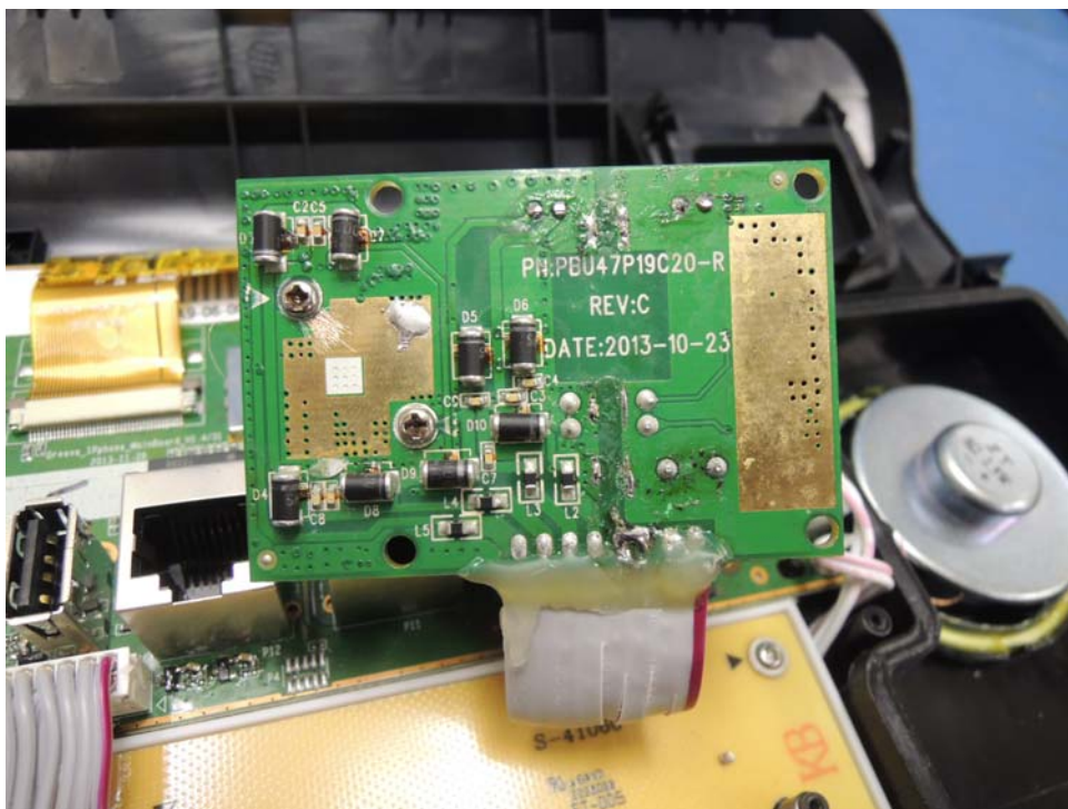
Base Unit PCB2 solder side (View 2)
