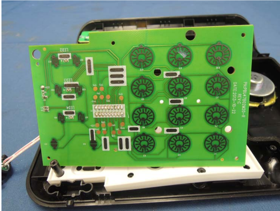
Base Unit Keypad side front side
