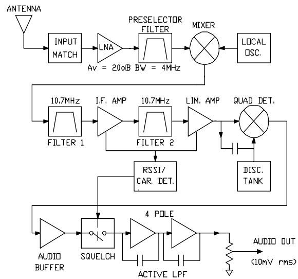
RF RECEIVER BLOCK DIAGRAM
