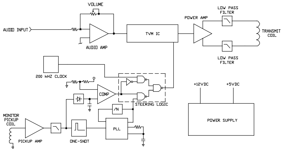
T.V.M. MAGNETIC TRANSMITTER BLOCK DIAGRAM
